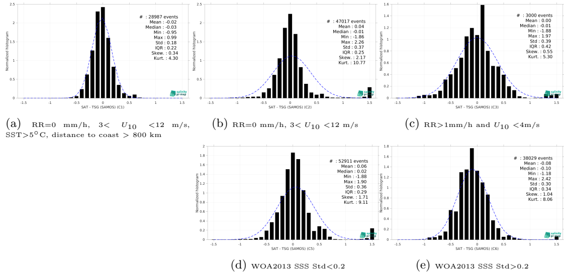
Figure 13: Normalized histogram of \Delta SSS (SMAP SSS L3 v5 - 8-Day running (RSS) - TSG (SAMOS)) for 5 different subdatasets corresponding to: RR=0 mm/h, 3 < U_{10} < 12 m/s, SST >5^\circ\text{C} , distance to coast > 800 km (a), RR=0 mm/h, 3 < U_{10} < 12 m/s (b), RR >1 mm/h and U_{10} < 4 m/s (c), WOA2013 SSS Std <0.2 (d), WOA2013 SSS Std >0.2 (e).
