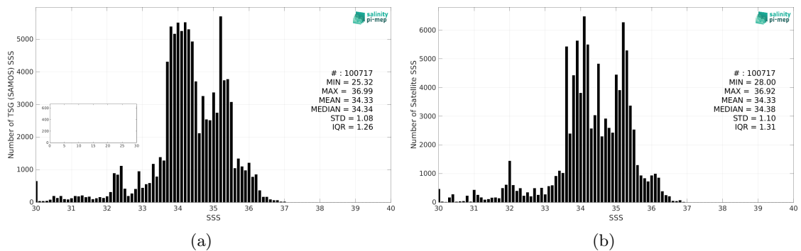
Figure 2: Histograms of SSS from TSG (SAMOS) (a) and SMAP SSS L3 v5 - 8-Day running (RSS) (b) considering all match-up pairs per bins of 0.1 over the Equatorial Ocean 10N-10S Pi-MEP region and for the full satellite product period.
