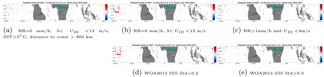
Figure 12: Temporal mean gridded over spatial boxes of size 1^\circ \times 1^\circ of \Delta SSS (SMAP SSS L3 v5 - 8-Day running (RSS) - TSG (SAMOS)) for 5 different subdatasets corresponding to: RR=0 mm/h, 3 < U_{10} < 12 m/s, SST >5^\circ\text{C} , distance to coast > 800 km (a), RR=0 mm/h, 3 < U_{10} < 12 m/s (b), RR >1 mm/h and U_{10} < 4 m/s (c), WOA2013 SSS Std <0.2 (d), WOA2013 SSS Std >0.2 (e).
