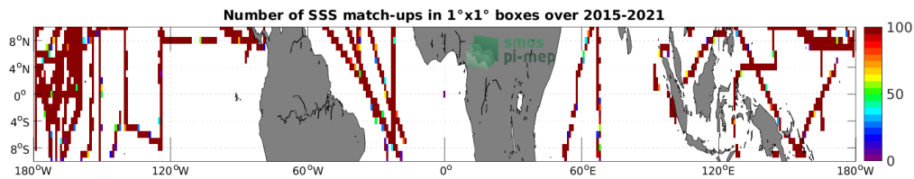
Figure 4: Number of SSS match-ups between TSG (SAMOS) SSS and the SMAP SSS L3 v5 - 8-Day running (RSS) SSS product for the Equatorial Ocean 10N-10S Pi-MEP region over 1^\circ \times 1^\circ boxes and for the full satellite product period.
