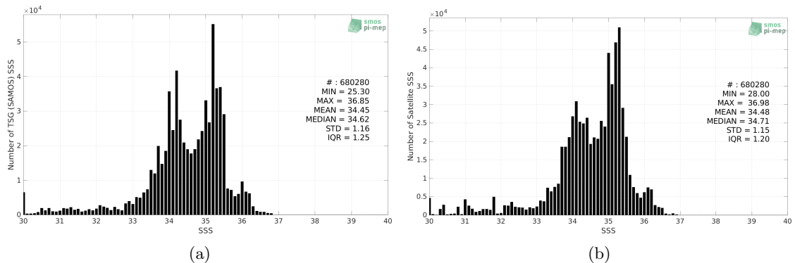
Figure 2: Histograms of SSS from TSG (SAMOS) (a) and SMAP SSS L3 v5 - 8-Day running (RSS) (b) considering all match-up pairs per bins of 0.1 over the Equatorial Ocean 10N-10S Pi-MEP region and for the full satellite product period.
