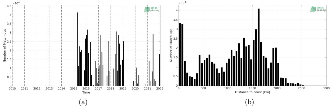
Figure 1: Number of match-ups between TSG (SAMOS) and SMAP SSS L3 v5 - 8-Day running (RSS) SSS as a function of time (a) and as function of the distance to coast (b) over the Equatorial Ocean 10N-10S Pi-MEP region and for the full satellite product period.
