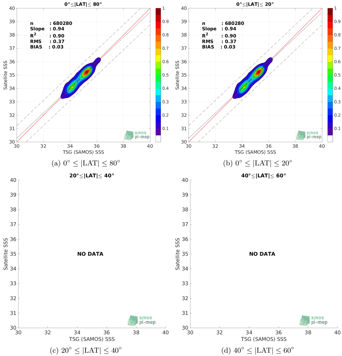
Figure 9: Contour maps of the concentration of SMAP SSS L3 v5 - 8-Day running (RSS) SSS (y-axis) versus TSG (SAMOS) SSS (x-axis) at match-up pairs for different latitude bands. For each plot, the red line shows x=y . The black thin and dashed lines indicate a linear fit through the data cloud and the \pm 95\% confidence levels, respectively. The number match-up pairs n , the slope and R^2 coefficient of the linear fit, the root mean square (RMS) and the mean bias between satellite and in situ data are indicated for each latitude band in each plots.
