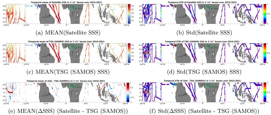
Figure 6: Temporal mean (left) and Std (right) of SSS from SMAP SSS L3 v5 - 8-Day running (RSS) (top), TSG (SAMOS) (middle), and of \Delta SSS (Satellite - TSG (SAMOS)). Only match-up pairs are used to generate these maps.
