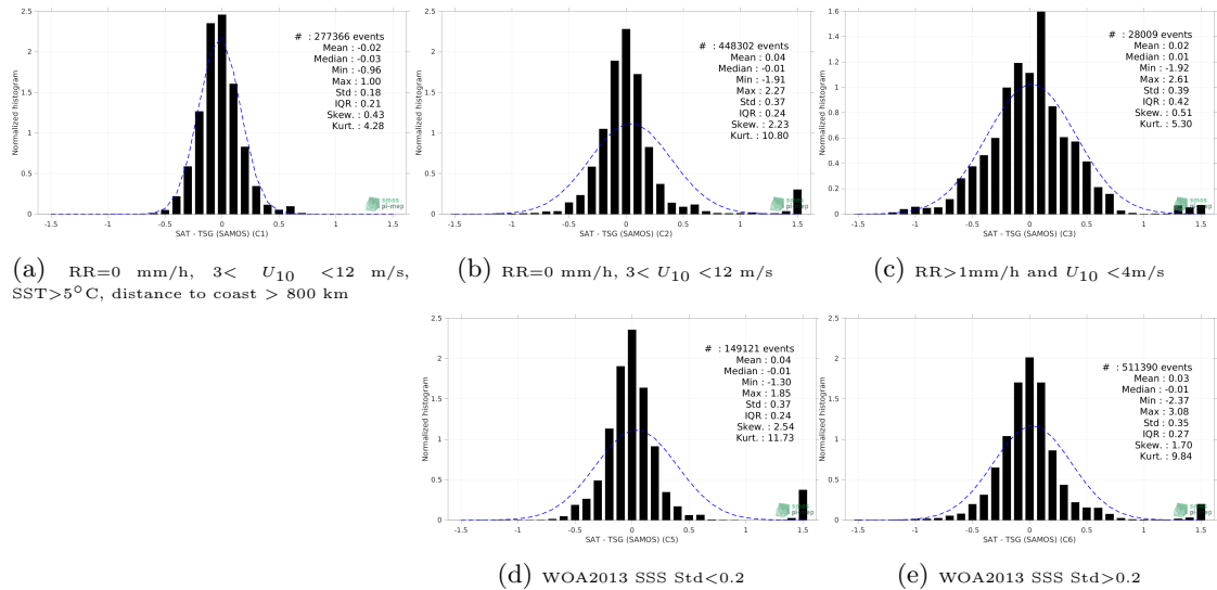
Figure 13: Normalized histogram of \Delta SSS (SMAP SSS L3 v5 - 8-Day running (RSS) - TSG (SAMOS)) for 5 different subdatasets corresponding to: RR=0 mm/h, 3 < U_{10} < 12 m/s, SST >5^\circ\text{C} , distance to coast > 800 km (a), RR=0 mm/h, 3 < U_{10} < 12 m/s (b), RR >1 mm/h and U_{10} < 4 m/s (c), WOA2013 SSS Std <0.2 (d), WOA2013 SSS Std >0.2 (e).
