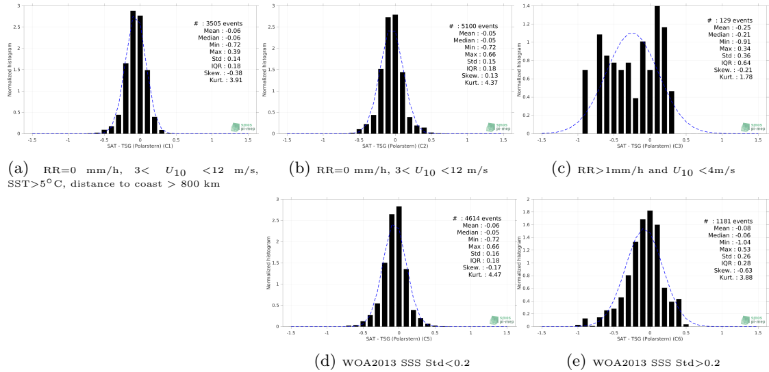
Figure 13: Normalized histogram of \Delta SSS (SMAP SSS L3 v5 - 8-Day running (RSS) - TSG (Polarstern)) for 5 different subdatasets corresponding to: RR=0 mm/h, 3 < U_{10} < 12 m/s, SST >5^\circ C, distance to coast > 800 km (a), RR=0 mm/h, 3 < U_{10} < 12 m/s (b), RR >1 mm/h and U_{10} < 4 m/s (c), WOA2013 SSS Std <0.2 (d), WOA2013 SSS Std >0.2 (e).
