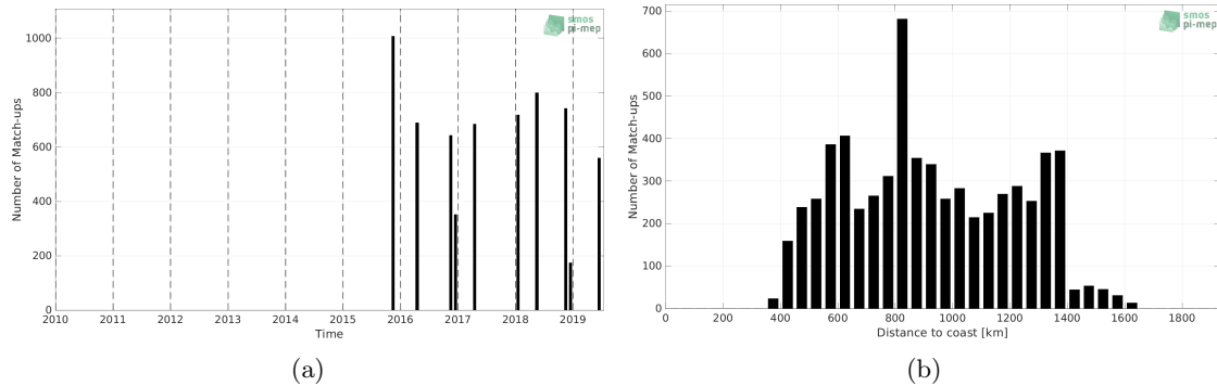
Figure 1: Number of match-ups between TSG (Polarstern) and SMAP SSS L3 v5 - 8-Day running (RSS) SSS as a function of time (a) and as function of the distance to coast (b) over the Equatorial Ocean 10N-10S Pi-MEP region and for the full satellite product period.
