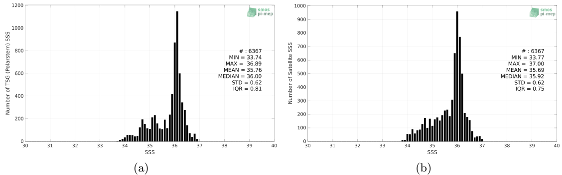
Figure 2: Histograms of SSS from TSG (Polarstern) (a) and SMAP SSS L3 v5 - 8-Day running (RSS) (b) considering all match-up pairs per bins of 0.1 over the Equatorial Ocean 10N-10S Pi-MEP region and for the full satellite product period.
