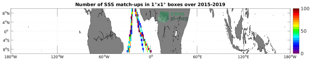
Figure 4: Number of SSS match-ups between TSG (Polarstern) SSS and the SMAP SSS L3 v5 - 8-Day running (RSS) SSS product for the Equatorial Ocean 10N-10S Pi-MEP region over 1^\circ \times 1^\circ boxes and for the full satellite product period.
