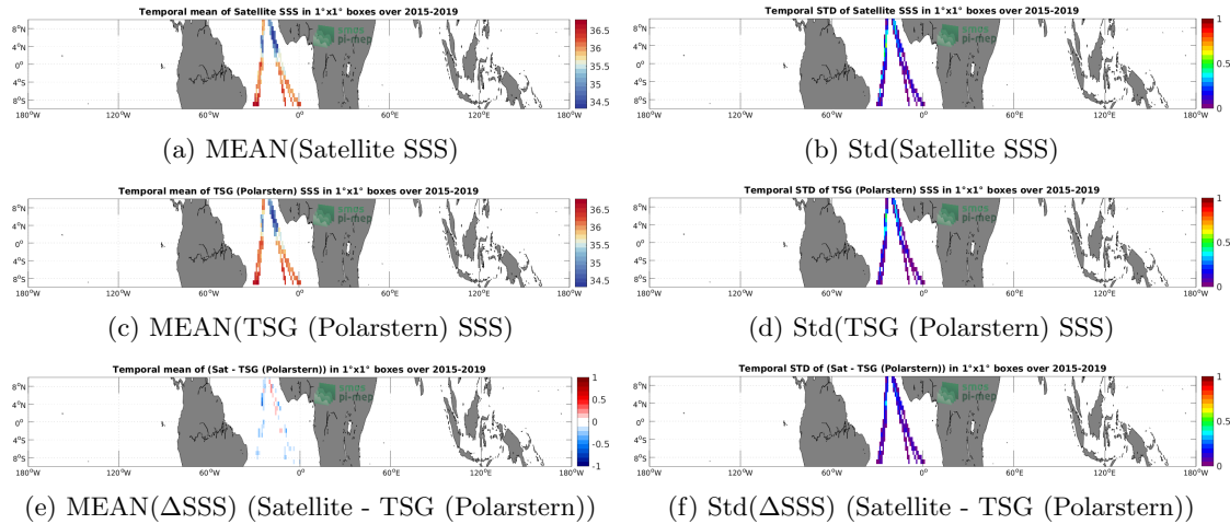
Figure 6: Temporal mean (left) and Std (right) of SSS from SMAP SSS L3 v5 - 8-Day running (RSS) (top), TSG (Polarstern) (middle), and of \Delta SSS (Satellite - TSG (Polarstern)). Only match-up pairs are used to generate these maps.
