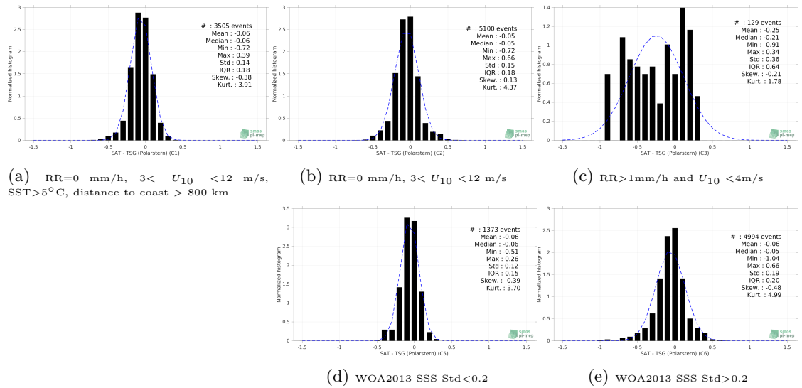
Figure 13: Normalized histogram of \Delta SSS (SMAP SSS L3 v5 - 8-Day running (RSS) - TSG (Polarstern)) for 5 different subdatasets corresponding to: RR=0 mm/h, 3 < U_{10} < 12 m/s, SST >5^\circ\text{C} , distance to coast > 800 km (a), RR=0 mm/h, 3 < U_{10} < 12 m/s (b), RR >1 mm/h and U_{10} < 4 m/s (c), WOA2013 SSS Std <0.2 (d), WOA2013 SSS Std >0.2 (e).
