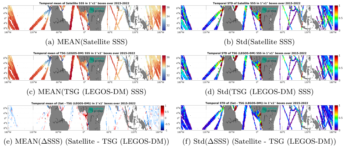
Figure 6: Temporal mean (left) and Std (right) of SSS from SMAP SSS L3 v5 - 8-Day running (RSS) (top), TSG (LEGOS-DM) (middle), and of \Delta SSS (Satellite - TSG (LEGOS-DM)). Only match-up pairs are used to generate these maps.
