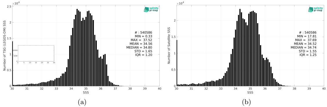
Figure 2: Histograms of SSS from TSG (LEGOS-DM) (a) and SMAP SSS L3 v5 - 8-Day running (RSS) (b) considering all match-up pairs per bins of 0.1 over the Equatorial Ocean 10N-10S Pi-MEP region and for the full satellite product period.
