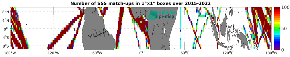
Figure 4: Number of SSS match-ups between TSG (LEGOS-DM) SSS and the SMAP SSS L3 v5 - 8-Day running (RSS) SSS product for the Equatorial Ocean 10N-10S Pi-MEP region over 1^\circ \times 1^\circ boxes and for the full satellite product period.
