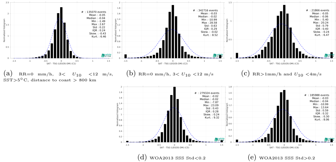
Figure 13: Normalized histogram of \Delta\text{SSS} (SMAP SSS L3 v5 - 8-Day running (RSS) - TSG (LEGOS-DM)) for 5 different subdatasets corresponding to: RR=0 mm/h, 3 < U_{10} < 12 m/s, SST >5^\circ\text{C} , distance to coast > 800 km (a), RR=0 mm/h, 3 < U_{10} < 12 m/s (b), RR >1 mm/h and U_{10} < 4 m/s (c), WOA2013 SSS Std <0.2 (d), WOA2013 SSS Std >0.2 (e).
