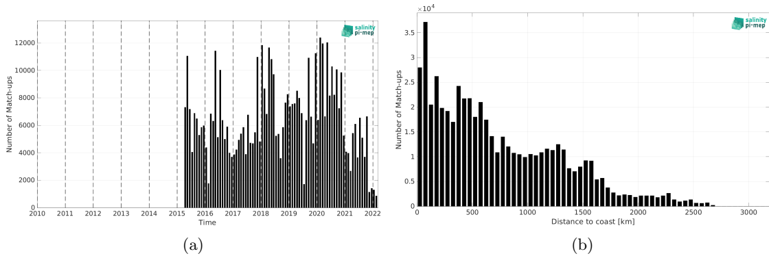
Figure 1: Number of match-ups between TSG (LEGOS-DM) and SMAP SSS L3 v5 - 8-Day running (RSS) SSS as a function of time (a) and as function of the distance to coast (b) over the Equatorial Ocean 10N-10S Pi-MEP region and for the full satellite product period.
