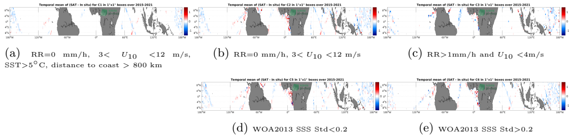
Figure 12: Temporal mean gridded over spatial boxes of size 1^\circ \times 1^\circ of \Delta SSS (SMAP SSS L3 v5 - 8-Day running (RSS) - TSG (LEGOS-DM)) for 5 different subdatasets corresponding to: RR=0 mm/h, 3 < U_{10} < 12 m/s, SST >5^\circ C, distance to coast > 800 km (a), RR=0 mm/h, 3 < U_{10} < 12 m/s (b), RR >1 mm/h and U_{10} < 4 m/s (c), WOA2013 SSS Std <0.2 (d), WOA2013 SSS Std >0.2 (e).
