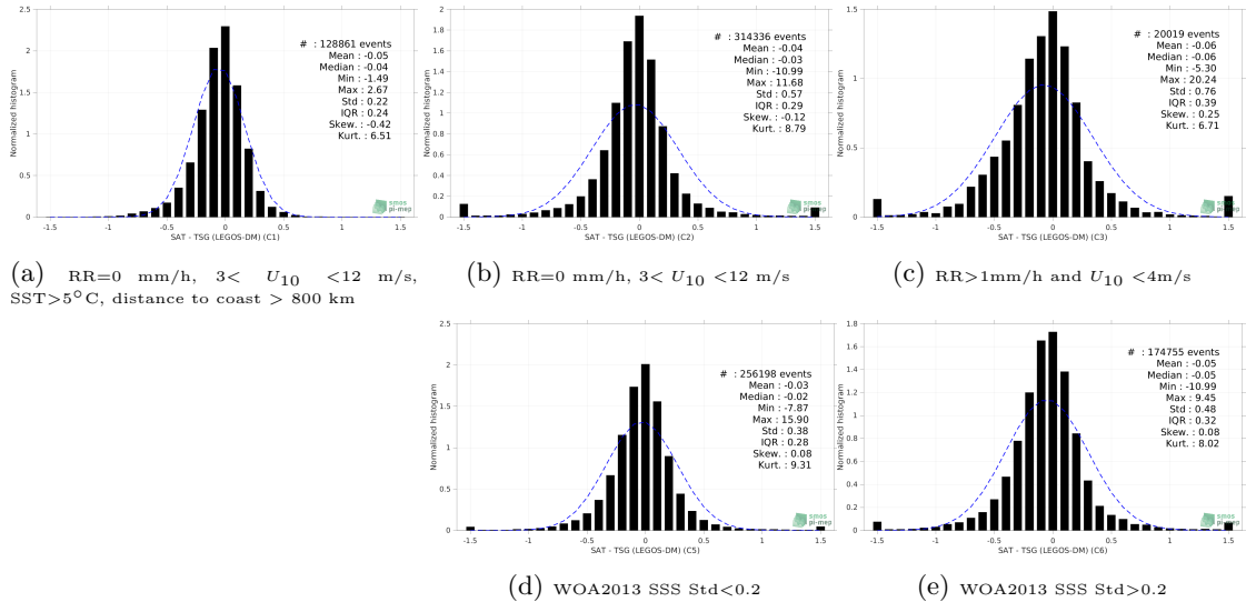
Figure 13: Normalized histogram of \Delta SSS (SMAP SSS L3 v5 - 8-Day running (RSS) - TSG (LEGOS-DM)) for 5 different subdatasets corresponding to: RR=0 mm/h, 3 < U_{10} < 12 m/s, SST >5^\circ C, distance to coast > 800 km (a), RR=0 mm/h, 3 < U_{10} < 12 m/s (b), RR >1 mm/h and U_{10} < 4 m/s (c), WOA2013 SSS Std <0.2 (d), WOA2013 SSS Std >0.2 (e).
