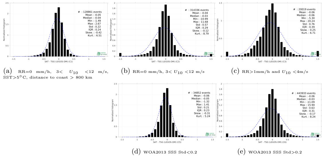
Figure 13: Normalized histogram of \Delta SSS (SMAP SSS L3 v5 - 8-Day running (RSS) - TSG (LEGOS-DM)) for 5 different subdatasets corresponding to: RR=0 mm/h, 3 < U_{10} < 12 m/s, SST >5^\circ\text{C} , distance to coast > 800 km (a), RR=0 mm/h, 3 < U_{10} < 12 m/s (b), RR >1 mm/h and U_{10} < 4 m/s (c), WOA2013 SSS Std <0.2 (d), WOA2013 SSS Std >0.2 (e).
