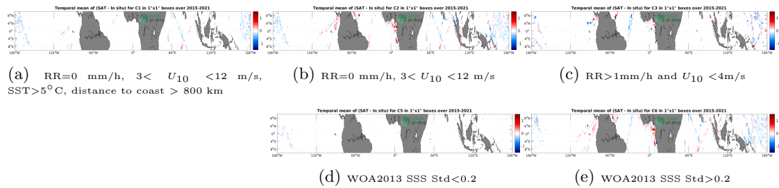
Figure 12: Temporal mean gridded over spatial boxes of size 1^\circ \times 1^\circ of \Delta SSS (SMAP SSS L3 v5 - 8-Day running (RSS) - TSG (LEGOS-DM)) for 5 different subdatasets corresponding to: RR=0 mm/h, 3 < U_{10} < 12 m/s, SST >5^\circ\text{C} , distance to coast > 800 km (a), RR=0 mm/h, 3 < U_{10} < 12 m/s (b), RR >1 mm/h and U_{10} < 4 m/s (c), WOA2013 SSS Std <0.2 (d), WOA2013 SSS Std >0.2 (e).
