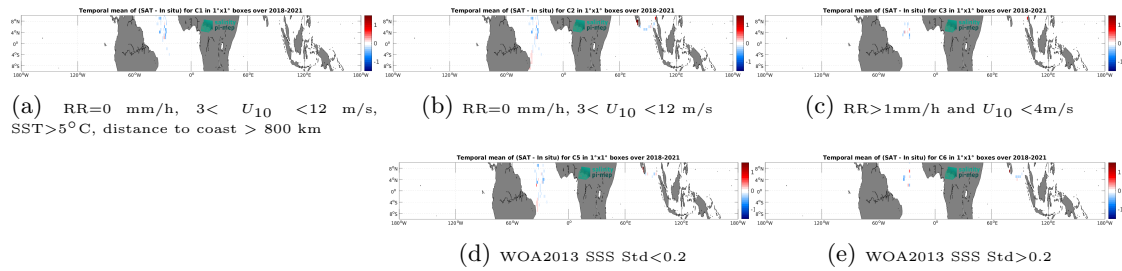
Figure 12: Temporal mean gridded over spatial boxes of size 1^\circ \times 1^\circ of \Delta\text{SSS} (SMAP SSS L3 v5 - 8-Day running (RSS) - TSG (GOSUD-Sailing-ship)) for 5 different subdatasets corresponding to: RR=0 mm/h, 3 < U_{10} < 12 m/s, SST>5°C, distance to coast > 800 km (a), RR=0 mm/h, 3 < U_{10} < 12 m/s (b), RR>1mm/h and U_{10} < 4 m/s (c), WOA2013 SSS Std<0.2 (d), WOA2013 SSS Std>0.2 (e).
