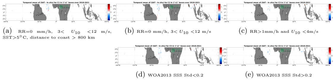
Figure 12: Temporal mean gridded over spatial boxes of size 1^\circ \times 1^\circ of \Delta SSS (SMAP SSS L3 v5 - 8-Day running (RSS) - TSG (GOSUD-Sailing-ship)) for 5 different subdatasets corresponding to: RR=0 mm/h, 3 < U_{10} < 12 m/s, SST>5°C, distance to coast > 800 km (a), RR=0 mm/h, 3 < U_{10} < 12 m/s (b), RR>1mm/h and U_{10} < 4 m/s (c), WOA2013 SSS Std<0.2 (d), WOA2013 SSS Std>0.2 (e).
