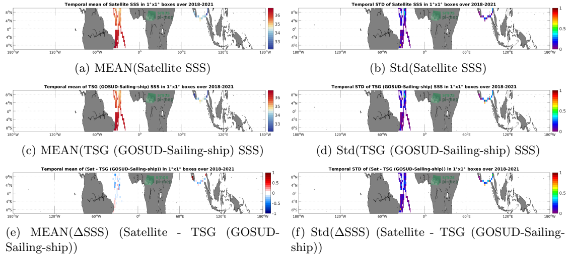
Figure 6: Temporal mean (left) and Std (right) of SSS from SMAP SSS L3 v5 - 8-Day running (RSS) (top), TSG (GOSUD-Sailing-ship) (middle), and of \Delta SSS (Satellite - TSG (GOSUD-Sailing-ship)). Only match-up pairs are used to generate these maps.
