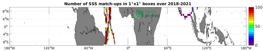
Figure 4: Number of SSS match-ups between TSG (GOSUD-Sailing-ship) SSS and the SMAP SSS L3 v5 - 8-Day running (RSS) SSS product for the Equatorial Ocean 10N-10S Pi-MEP region over 1^\circ \times 1^\circ boxes and for the full satellite product period.
