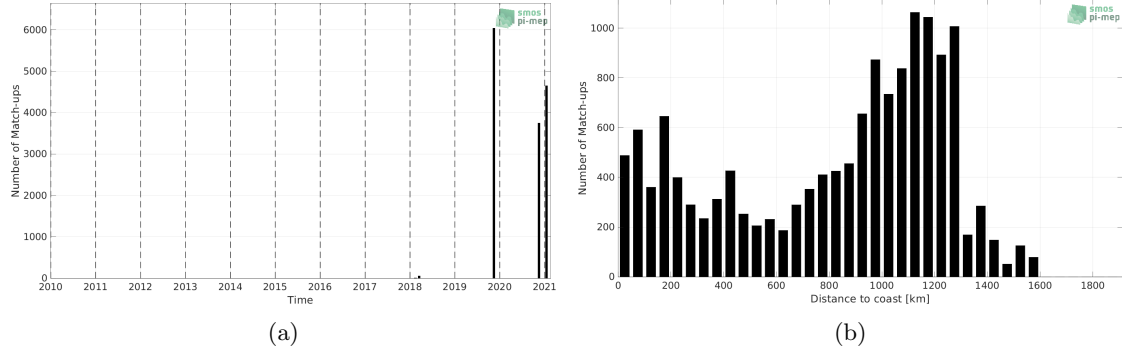
Figure 1: Number of match-ups between TSG (GOSUD-Sailing-ship) and SMAP SSS L3 v5 - 8-Day running (RSS) SSS as a function of time (a) and as function of the distance to coast (b) over the Equatorial Ocean 10N-10S Pi-MEP region and for the full satellite product period.
