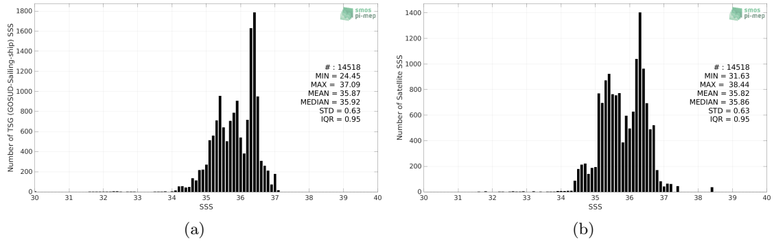
Figure 2: Histograms of SSS from TSG (GOSUD-Sailing-ship) (a) and SMAP SSS L3 v5 - 8-Day running (RSS) (b) considering all match-up pairs per bins of 0.1 over the Equatorial Ocean 10N-10S Pi-MEP region and for the full satellite product period.
