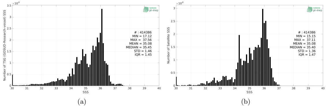
Figure 2: Histograms of SSS from TSG (GOSUD-Research-vessel) (a) and SMAP SSS L3 v5 - 8-Day running (RSS) (b) considering all match-up pairs per bins of 0.1 over the Equatorial Ocean 10N-10S Pi-MEP region and for the full satellite product period.
