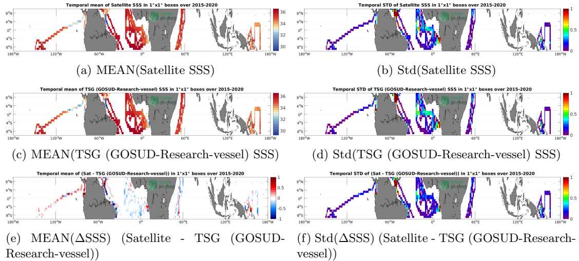
Figure 6: Temporal mean (left) and Std (right) of SSS from SMAP SSS L3 v5 - 8-Day running (RSS) (top), TSG (GOSUD-Research-vessel) (middle), and of \Delta SSS (Satellite - TSG (GOSUD-Research-vessel)). Only match-up pairs are used to generate these maps.
