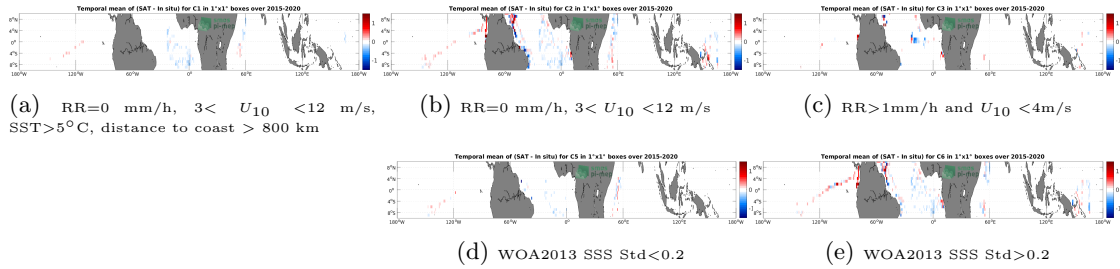
Figure 12: Temporal mean gridded over spatial boxes of size 1^\circ \times 1^\circ of \Delta SSS (SMAP SSS L3 v5 - 8-Day running (RSS) - TSG (GOSUD-Research-vessel)) for 5 different subdatasets corresponding to: RR=0 mm/h, 3 < U_{10} < 12 m/s, SST>5°C, distance to coast > 800 km (a), RR=0 mm/h, 3 < U_{10} < 12 m/s (b), RR>1mm/h and U_{10} < 4 m/s (c), WOA2013 SSS Std<0.2 (d), WOA2013 SSS Std>0.2 (e).
