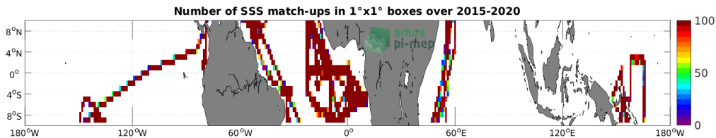
Figure 4: Number of SSS match-ups between TSG (GOSUD-Research-vessel) SSS and the SMAP SSS L3 v5 - 8-Day running (RSS) SSS product for the Equatorial Ocean 10N-10S Pi-MEP region over 1^\circ \times 1^\circ boxes and for the full satellite product period.
