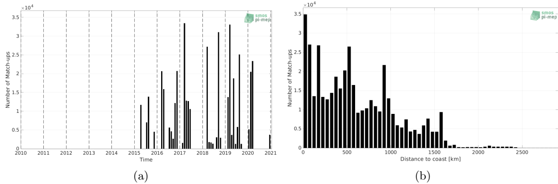
Figure 1: Number of match-ups between TSG (GOSUD-Research-vessel) and SMAP SSS L3 v5 - 8-Day running (RSS) SSS as a function of time (a) and as function of the distance to coast (b) over the Equatorial Ocean 10N-10S Pi-MEP region and for the full satellite product period.
