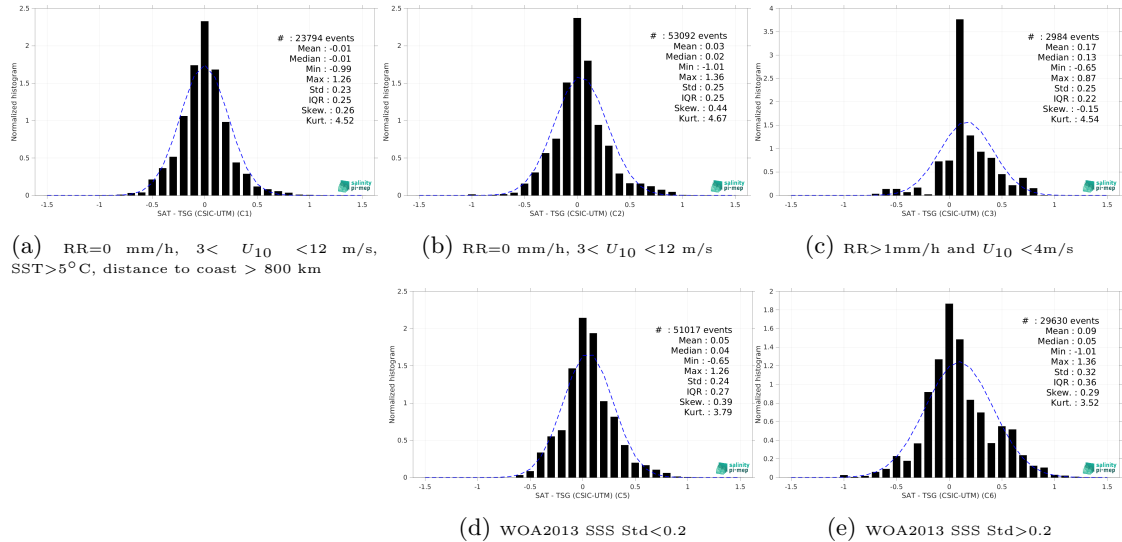
Figure 13: Normalized histogram of \Delta SSS (SMAP SSS L3 v5 - 8-Day running (RSS) - TSG (CSIC-UTM)) for 5 different subdatasets corresponding to: RR=0 mm/h, 3 < U_{10} < 12 m/s, SST >5^\circ C, distance to coast > 800 km (a), RR=0 mm/h, 3 < U_{10} < 12 m/s (b), RR >1 mm/h and U_{10} < 4 m/s (c), WOA2013 SSS Std <0.2 (d), WOA2013 SSS Std >0.2 (e).
