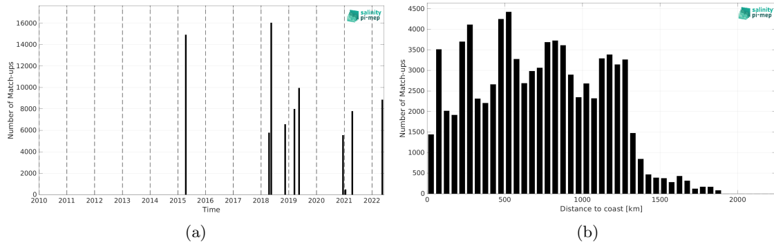
Figure 1: Number of match-ups between TSG (CSIC-UTM) and SMAP SSS L3 v5 - 8-Day running (RSS) SSS as a function of time (a) and as function of the distance to coast (b) over the Equatorial Ocean 10N-10S Pi-MEP region and for the full satellite product period.
