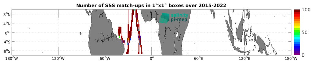
Figure 4: Number of SSS match-ups between TSG (CSIC-UTM) SSS and the SMAP SSS L3 v5 - 8-Day running (RSS) SSS product for the Equatorial Ocean 10N-10S Pi-MEP region over 1^\circ \times 1^\circ boxes and for the full satellite product period.
