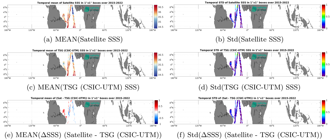
Figure 6: Temporal mean (left) and Std (right) of SSS from SMAP SSS L3 v5 - 8-Day running (RSS) (top), TSG (CSIC-UTM) (middle), and of \Delta SSS (Satellite - TSG (CSIC-UTM)). Only match-up pairs are used to generate these maps.
