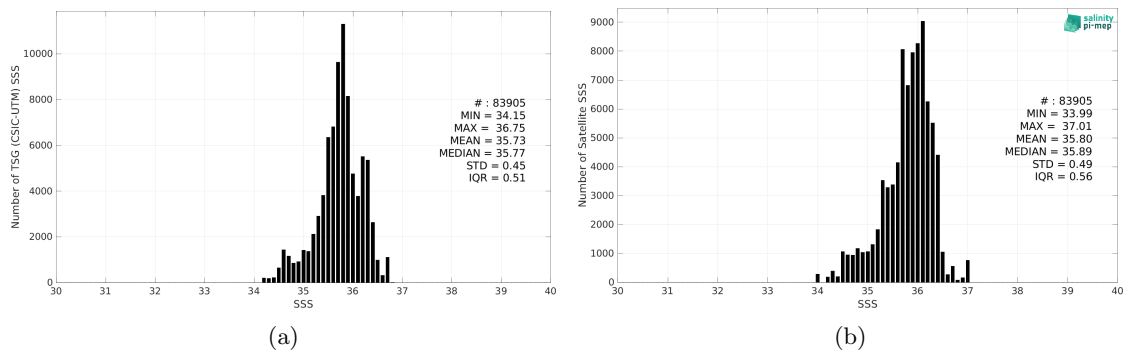
Figure 2: Histograms of SSS from TSG (CSIC-UTM) (a) and SMAP SSS L3 v5 - 8-Day running (RSS) (b) considering all match-up pairs per bins of 0.1 over the Equatorial Ocean 10N-10S Pi-MEP region and for the full satellite product period.
