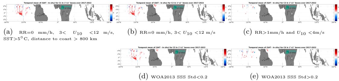
Figure 12: Temporal mean gridded over spatial boxes of size 1^\circ \times 1^\circ of \Delta SSS (SMAP SSS L3 v5 - 8-Day running (RSS) - Saildrone) for 5 different subdatasets corresponding to:RR=0 mm/h, 3 < U_{10} < 12 m/s, SST > 5^\circ C , distance to coast > 800 km (a), RR=0 mm/h, 3 < U_{10} < 12 m/s (b), RR >1 mm/h and U_{10} < 4 m/s (c), WOA2013 SSS Std <0.2 (d), WOA2013 SSS Std >0.2 (e).
