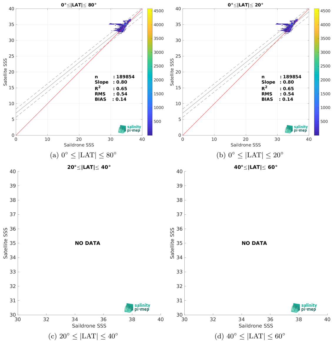
Figure 9: Contour maps of the concentration of SMAP SSS L3 v5 - 8-Day running (RSS) SSS (y-axis) versus Sairdron SSS (x-axis) at match-up pairs for different latitude bands. For each plot, the red line shows x=y . The black thin and dashed lines indicate a linear fit through the data cloud and the \pm 95\% confidence levels, respectively. The number match-up pairs n , the slope and R^2 coefficient of the linear fit, the root mean square (RMS) and the mean bias between satellite and in situ data are indicated for each latitude band in each plots.
