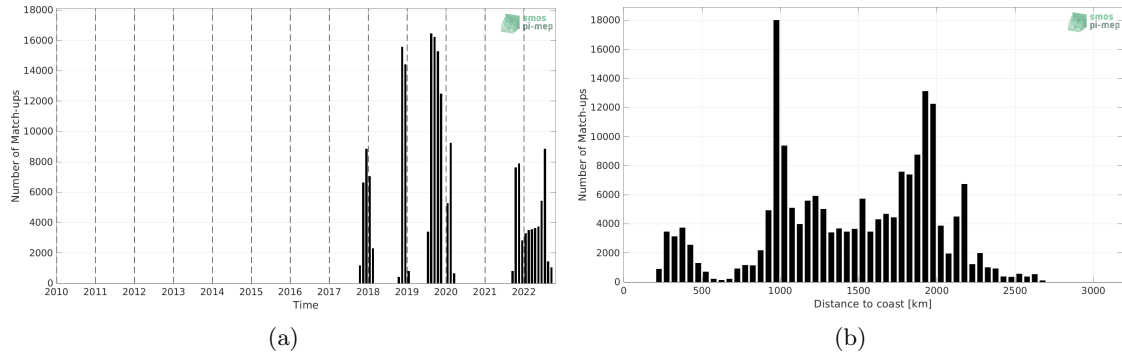
Figure 1: Number of match-ups between Saildrone and SMAP SSS L3 v5 - 8-Day running (RSS) SSS as a function of time (a) and as function of the distance to coast (b) over the Equatorial Ocean 10N-10S Pi-MEP region and for the full satellite product period.
