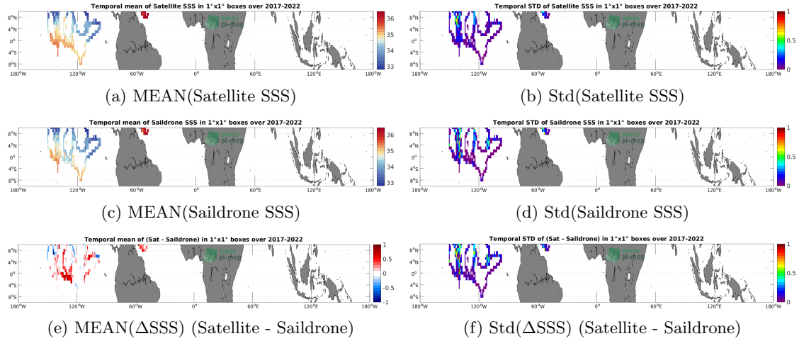
Figure 6: Temporal mean (left) and Std (right) of SSS from SMAP SSS L3 v5 - 8-Day running (RSS) (top), Saildrone (middle), and of \Delta SSS (Satellite - Saildrone). Only match-up pairs are used to generate these maps.
