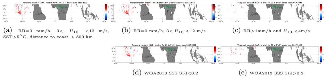
Figure 12: Temporal mean gridded over spatial boxes of size 1^\circ \times 1^\circ of \Delta SSS (SMAP SSS L3 v5 - 8-Day running (RSS) - Saildrone) for 5 different subdatasets corresponding to: RR=0 mm/h, 3 < U_{10} < 12 m/s, SST > 5^\circ C , distance to coast > 800 km (a), RR=0 mm/h, 3 < U_{10} < 12 m/s (b), RR > 1 mm/h and U_{10} < 4 m/s (c), WOA2013 SSS Std < 0.2 (d), WOA2013 SSS Std > 0.2 (e).
