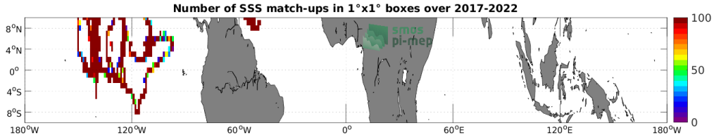
Figure 4: Number of SSS match-ups between Saildrone SSS and the SMAP SSS L3 v5 - 8-Day running (RSS) SSS product for the Equatorial Ocean 10N-10S Pi-MEP region over 1^\circ \times 1^\circ boxes and for the full satellite product period.
