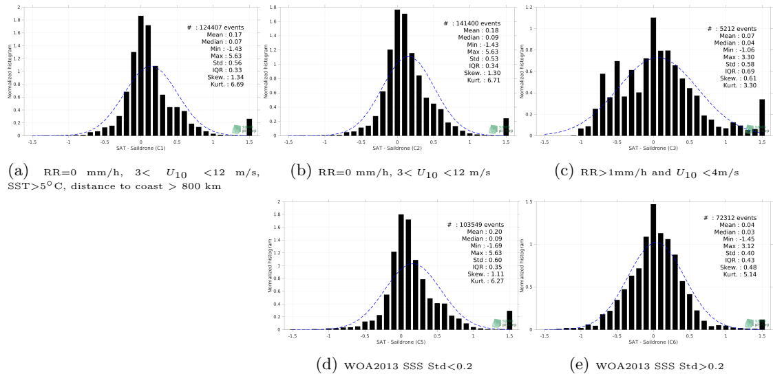
Figure 13: Normalized histogram of \Delta SSS (SMAP SSS L3 v5 - 8-Day running (RSS) - Saildrone) for 5 different subdatasets corresponding to: RR=0 mm/h, 3 < U_{10} < 12 m/s, SST > 5^\circ C , distance to coast > 800 km (a), RR=0 mm/h, 3 < U_{10} < 12 m/s (b), RR > 1 mm/h and U_{10} < 4 m/s (c), WOA2013 SSS Std < 0.2 (d), WOA2013 SSS Std > 0.2 (e).
