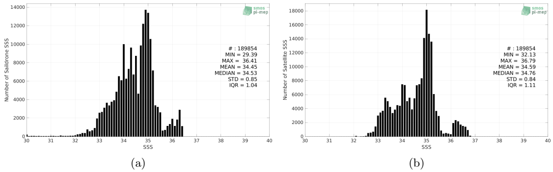
Figure 2: Histograms of SSS from Saildrone (a) and SMAP SSS L3 v5 - 8-Day running (RSS) (b) considering all match-up pairs per bins of 0.1 over the Equatorial Ocean 10N-10S Pi-MEP region and for the full satellite product period.
