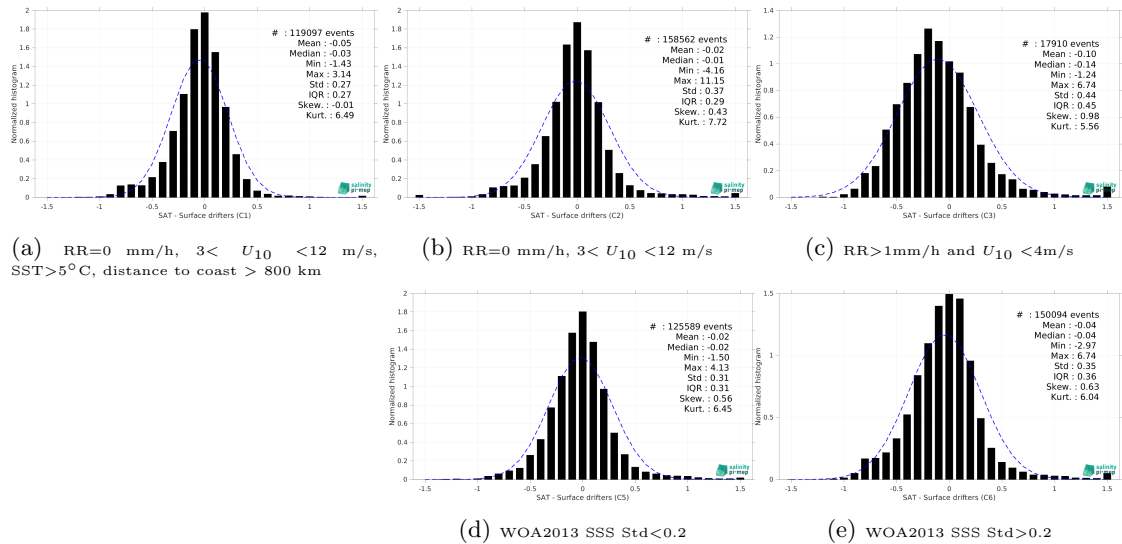
Figure 12: Normalized histogram of \Delta SSS (SMAP SSS L3 v5 - 8-Day running (RSS) - Surface drifters) for 5 different subdatasets corresponding to: RR=0 mm/h, 3 < U_{10} < 12 m/s, SST >5^\circ C, distance to coast > 800 km (a), RR=0 mm/h, 3 < U_{10} < 12 m/s (b), RR >1 mm/h and U_{10} < 4 m/s (c), WOA2013 SSS Std <0.2 (d), WOA2013 SSS Std >0.2 (e).
