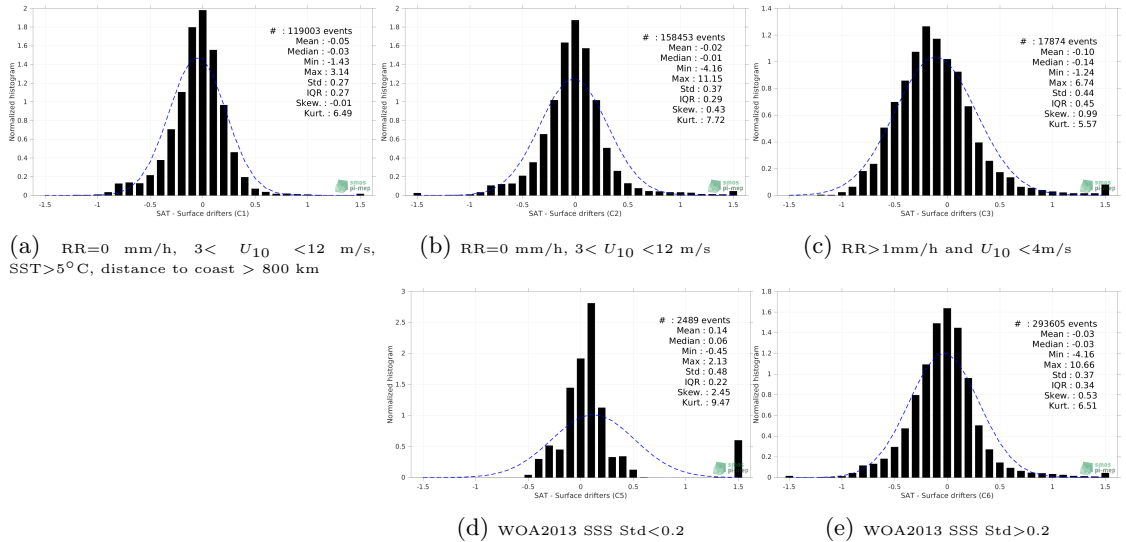
Figure 12: Normalized histogram of \Delta SSS (SMAP SSS L3 v5 - 8-Day running (RSS) - Surface drifters) for 5 different subdatasets corresponding to: RR=0 mm/h, 3 < U_{10} < 12 m/s, SST>5°C, distance to coast > 800 km (a), RR=0 mm/h, 3 < U_{10} < 12 m/s (b), RR>1mm/h and U_{10} < 4 m/s (c), WOA2013 SSS Std<0.2 (d), WOA2013 SSS Std>0.2 (e).
