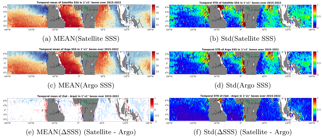
Figure 6: Temporal mean (left) and Std (right) of SSS from SMAP SSS L3 v5 - 8-Day running (RSS) (top), Argo (middle), and of \Delta SSS (Satellite - Argo). Only match-up pairs are used to generate these maps.
