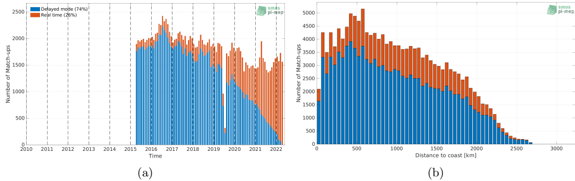
Figure 1: Number of match-ups between Argo and SMAP SSS L3 v5 - 8-Day running (RSS) SSS as a function of time (a) and as function of the distance to coast (b) over the Equatorial Ocean 10N-10S Pi-MEP region and for the full satellite product period.
