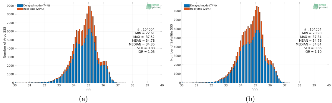
Figure 2: Histograms of SSS from Argo (a) and SMAP SSS L3 v5 - 8-Day running (RSS) (b) considering all match-up pairs per bins of 0.1 over the Equatorial Ocean 10N-10S Pi-MEP region and for the full satellite product period.
