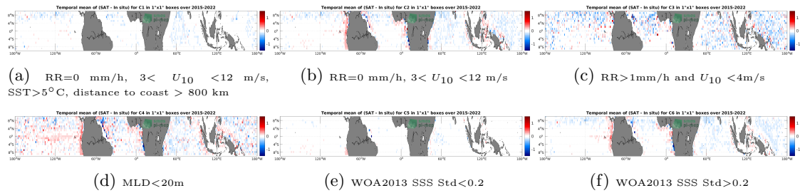
Figure 12: Temporal mean gridded over spatial boxes of size 1^\circ \times 1^\circ of \Delta SSS (SMAP SSS L3 v5 - 8-Day running (RSS) - Argo) for 6 different subdatasets corresponding to:RR=0 mm/h, 3 < U_{10} < 12 m/s, SST >5^\circ C, distance to coast > 800 km (a), RR=0 mm/h, 3 < U_{10} < 12 m/s (b), RR >1 mm/h and U_{10} < 4 m/s (c),MLD <20 m (d),WOA2013 SSS Std <0.2 (e),WOA2013 SSS Std >0.2 (f).
