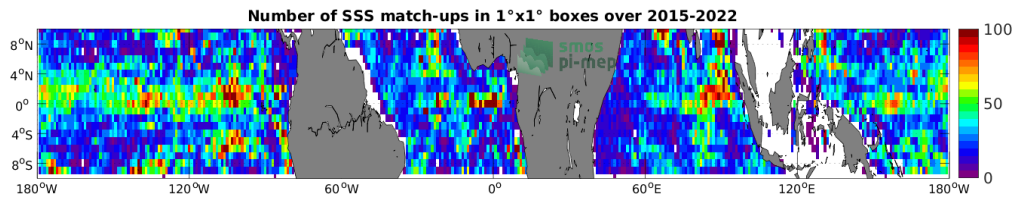
Figure 4: Number of SSS match-ups between Argo SSS and the SMAP SSS L3 v5 - 8-Day running (RSS) SSS product for the Equatorial Ocean 10N-10S Pi-MEP region over 1^\circ \times 1^\circ boxes and for the full satellite product period.
