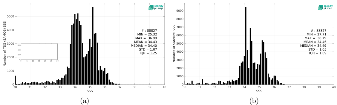
Figure 2: Histograms of SSS from TSG (SAMOS) (a) and SMAP SSS L3 v5 - Monthly (RSS) (b) considering all match-up pairs per bins of 0.1 over the Equatorial Ocean 10N-10S Pi-MEP region and for the full satellite product period.
