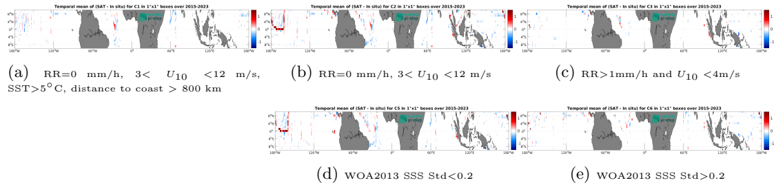
Figure 12: Temporal mean gridded over spatial boxes of size 1^\circ \times 1^\circ of \Delta SSS (SMAP SSS L3 v5 - Monthly (RSS) - TSG (SAMOS)) for 5 different subdatasets corresponding to:RR=0 mm/h, 3 < U_{10} < 12 m/s, SST >5^\circ\text{C} , distance to coast > 800 km (a), RR=0 mm/h, 3 < U_{10} < 12 m/s (b), RR >1 mm/h and U_{10} < 4 m/s (c), WOA2013 SSS Std <0.2 (d), WOA2013 SSS Std >0.2 (e).
