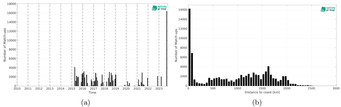
Figure 1: Number of match-ups between TSG (SAMOS) and SMAP SSS L3 v5 - Monthly (RSS) SSS as a function of time (a) and as function of the distance to coast (b) over the Equatorial Ocean 10N-10S Pi-MEP region and for the full satellite product period.
