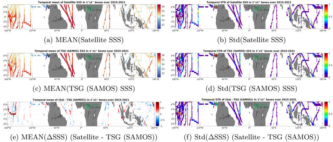
Figure 6: Temporal mean (left) and Std (right) of SSS from SMAP SSS L3 v5 - Monthly (RSS) (top), TSG (SAMOS) (middle), and of \Delta SSS (Satellite - TSG (SAMOS)). Only match-up pairs are used to generate these maps.
