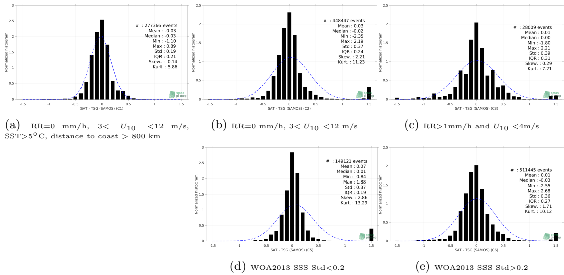
Figure 13: Normalized histogram of \Delta SSS (SMAP SSS L3 v5 - Monthly (RSS) - TSG (SAMOS)) for 5 different subdatasets corresponding to: RR=0 mm/h, 3 < U_{10} < 12 m/s, SST > 5^\circ C , distance to coast > 800 km (a), RR=0 mm/h, 3 < U_{10} < 12 m/s (b), RR>1mm/h and U_{10} < 4 m/s (c), WOA2013 SSS Std<0.2 (d), WOA2013 SSS Std>0.2 (e).
