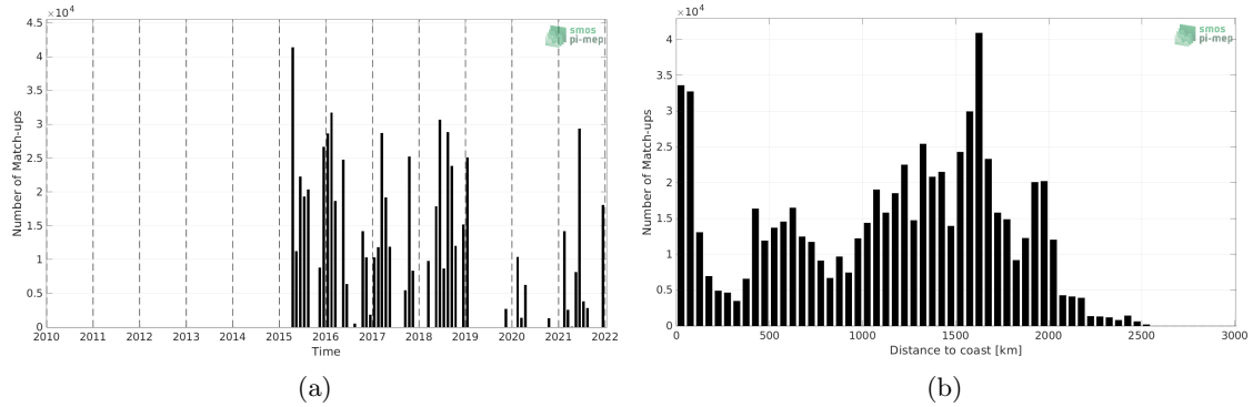
Figure 1: Number of match-ups between TSG (SAMOS) and SMAP SSS L3 v5 - Monthly (RSS) SSS as a function of time (a) and as function of the distance to coast (b) over the Equatorial Ocean 10N-10S Pi-MEP region and for the full satellite product period.
