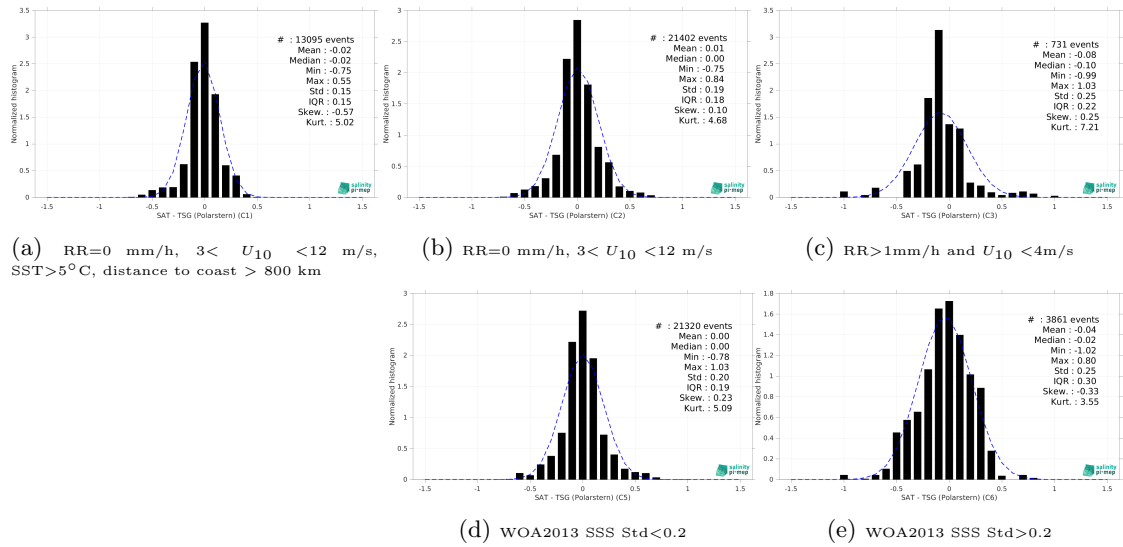
Figure 13: Normalized histogram of \Delta SSS (SMAP SSS L3 v5 - Monthly (RSS) - TSG (Polarstern)) for 5 different subdatasets corresponding to: RR=0 mm/h, 3 < U_{10} < 12 m/s, SST >5^\circ\text{C} , distance to coast > 800 km (a), RR=0 mm/h, 3 < U_{10} < 12 m/s (b), RR >1 mm/h and U_{10} < 4 m/s (c), WOA2013 SSS Std <0.2 (d), WOA2013 SSS Std >0.2 (e).
