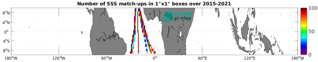
Figure 4: Number of SSS match-ups between TSG (Polarstern) SSS and the SMAP SSS L3 v5 - Monthly (RSS) SSS product for the Equatorial Ocean 10N-10S Pi-MEP region over 1^\circ \times 1^\circ boxes and for the full satellite product period.
