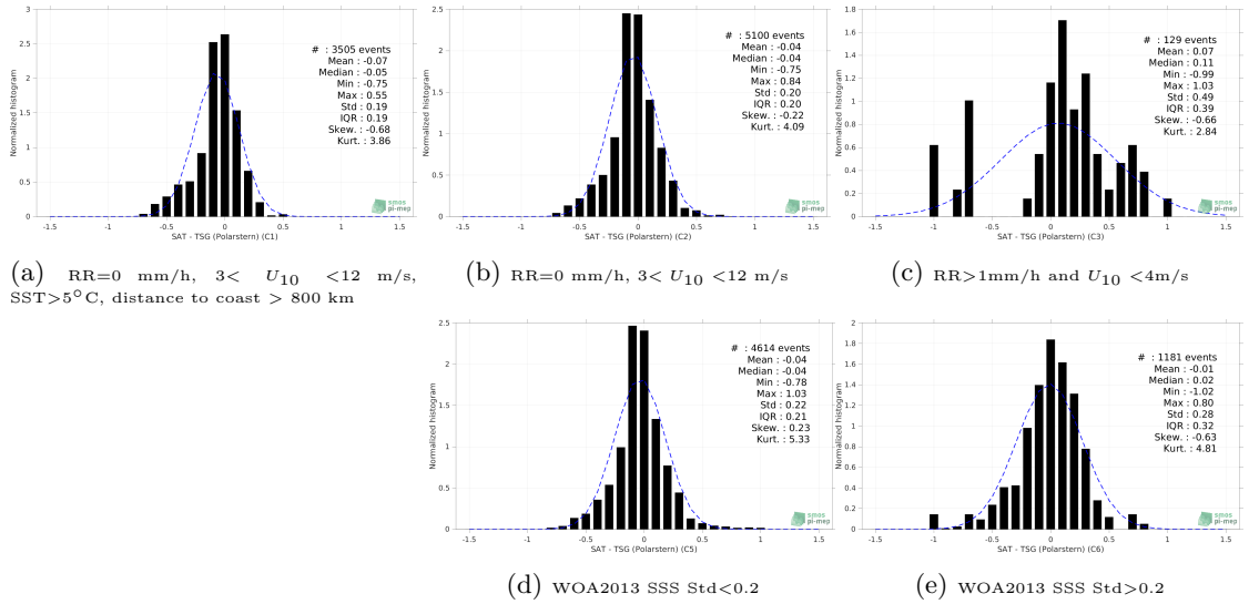
Figure 13: Normalized histogram of \Delta SSS (SMAP SSS L3 v5 - Monthly (RSS) - TSG (Polarstern)) for 5 different subdatasets corresponding to: RR=0 mm/h, 3 < U_{10} < 12 m/s, SST >5^\circ C , distance to coast > 800 km (a), RR=0 mm/h, 3 < U_{10} < 12 m/s (b), RR >1 mm/h and U_{10} < 4 m/s (c), WOA2013 SSS Std <0.2 (d), WOA2013 SSS Std >0.2 (e).
