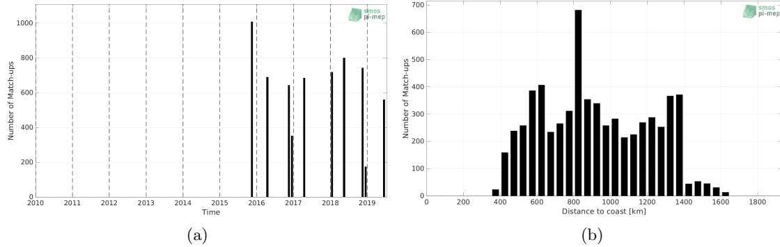
Figure 1: Number of match-ups between TSG (Polarstern) and SMAP SSS L3 v5 - Monthly (RSS) SSS as a function of time (a) and as function of the distance to coast (b) over the Equatorial Ocean 10N-10S Pi-MEP region and for the full satellite product period.
