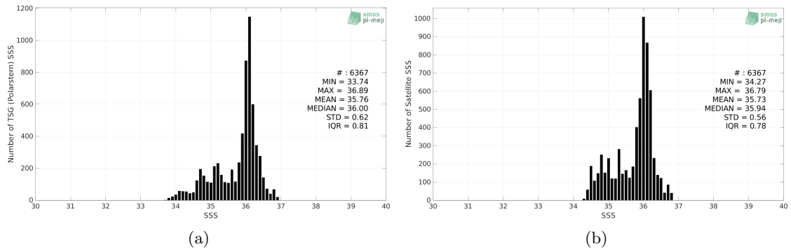
Figure 2: Histograms of SSS from TSG (Polarstern) (a) and SMAP SSS L3 v5 - Monthly (RSS) (b) considering all match-up pairs per bins of 0.1 over the Equatorial Ocean 10N-10S Pi-MEP region and for the full satellite product period.
