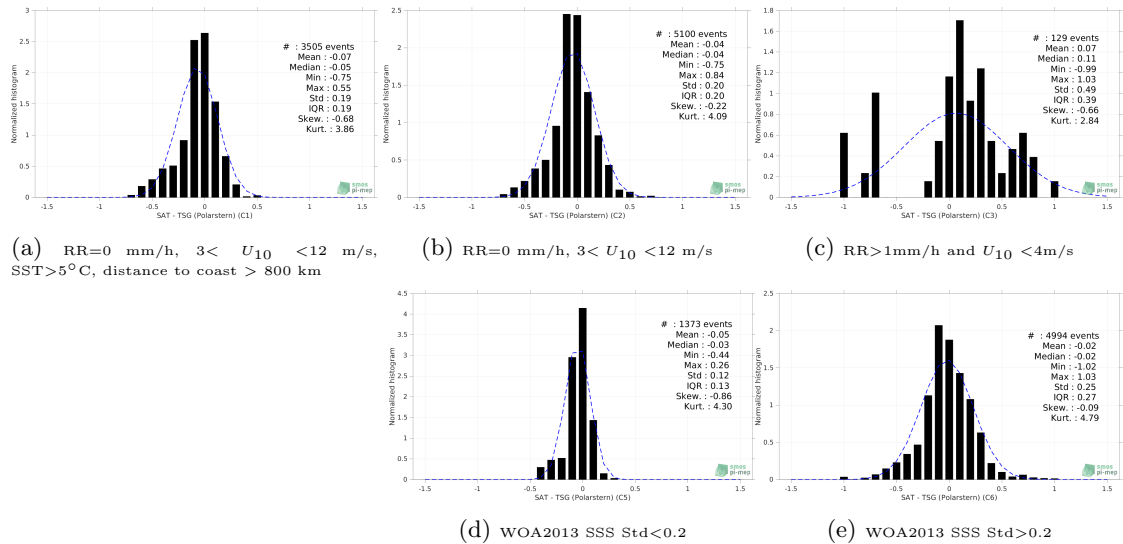
Figure 13: Normalized histogram of \Delta SSS (SMAP SSS L3 v5 - Monthly (RSS) - TSG (Polarstern)) for 5 different subdatasets corresponding to: RR=0 mm/h, 3 < U_{10} < 12 m/s, SST>5°C, distance to coast > 800 km (a), RR=0 mm/h, 3 < U_{10} < 12 m/s (b), RR>1mm/h and U_{10} < 4 m/s (c), WOA2013 SSS Std<0.2 (d), WOA2013 SSS Std>0.2 (e).
