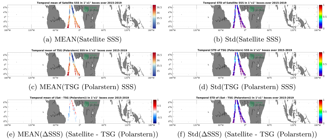
Figure 6: Temporal mean (left) and Std (right) of SSS from SMAP SSS L3 v5 - Monthly (RSS) (top), TSG (Polarstern) (middle), and of \Delta SSS (Satellite - TSG (Polarstern)). Only match-up pairs are used to generate these maps.
