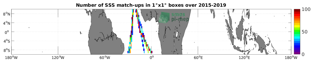
Figure 4: Number of SSS match-ups between TSG (Polarstern) SSS and the SMAP SSS L3 v5 - Monthly (RSS) SSS product for the Equatorial Ocean 10N-10S Pi-MEP region over 1^\circ \times 1^\circ boxes and for the full satellite product period.
