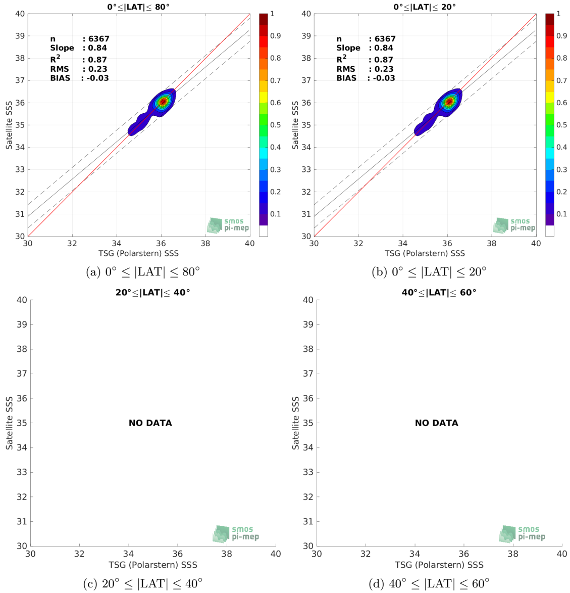
Figure 9: Contour maps of the concentration of SMAP SSS L3 v5 - Monthly (RSS) SSS (y-axis) versus TSG (Polarstern) SSS (x-axis) at match-up pairs for different latitude bands. For each plot, the red line shows x=y . The black thin and dashed lines indicate a linear fit through the data cloud and the \pm 95\% confidence levels, respectively. The number match-up pairs n , the slope and R^2 coefficient of the linear fit, the root mean square (RMS) and the mean bias between satellite and in situ data are indicated for each latitude band in each plots.
