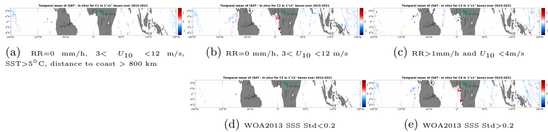
Figure 12: Temporal mean gridded over spatial boxes of size 1^\circ \times 1^\circ of \Delta SSS (SMAP SSS L3 v5 - Monthly (RSS) - TSG (LEGOS-DM)) for 5 different subdatasets corresponding to:RR=0 mm/h, 3 < U_{10} < 12 m/s, SST >5^\circ C, distance to coast > 800 km (a), RR=0 mm/h, 3 < U_{10} < 12 m/s (b), RR >1 mm/h and U_{10} < 4 m/s (c), WOA2013 SSS Std <0.2 (d), WOA2013 SSS Std >0.2 (e).
