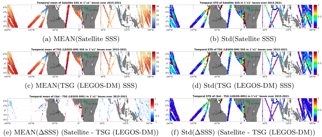
Figure 6: Temporal mean (left) and Std (right) of SSS from SMAP SSS L3 v5 - Monthly (RSS) (top), TSG (LEGOS-DM) (middle), and of \Delta SSS (Satellite - TSG (LEGOS-DM)). Only match-up pairs are used to generate these maps.
