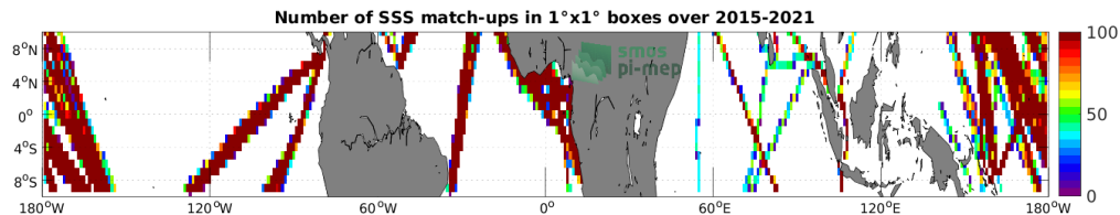
Figure 4: Number of SSS match-ups between TSG (LEGOS-DM) SSS and the SMAP SSS L3 v5 - Monthly (RSS) SSS product for the Equatorial Ocean 10N-10S Pi-MEP region over 1^\circ \times 1^\circ boxes and for the full satellite product period.
