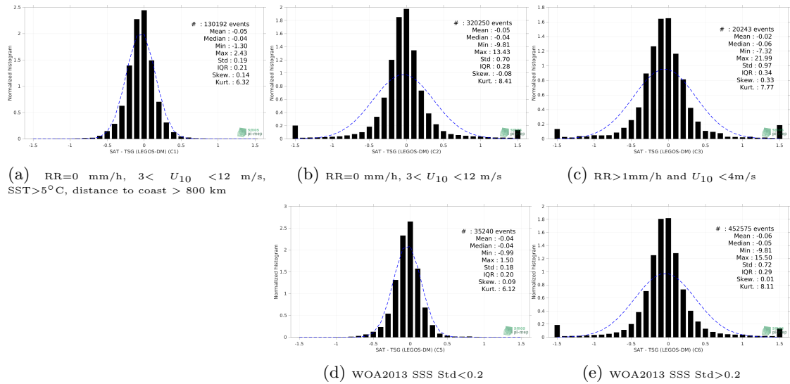
Figure 13: Normalized histogram of \Delta SSS (SMAP SSS L3 v5 - Monthly (RSS) - TSG (LEGOS-DM)) for 5 different subdatasets corresponding to: RR=0 mm/h, 3 < U_{10} < 12 m/s, SST >5^\circ C, distance to coast > 800 km (a), RR=0 mm/h, 3 < U_{10} < 12 m/s (b), RR >1 mm/h and U_{10} < 4 m/s (c), WOA2013 SSS Std <0.2 (d), WOA2013 SSS Std >0.2 (e).
