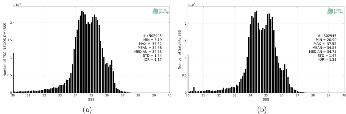
Figure 2: Histograms of SSS from TSG (LEGOS-DM) (a) and SMAP SSS L3 v5 - Monthly (RSS) (b) considering all match-up pairs per bins of 0.1 over the Equatorial Ocean 10N-10S Pi-MEP region and for the full satellite product period.
