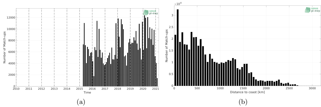
Figure 1: Number of match-ups between TSG (LEGOS-DM) and SMAP SSS L3 v5 - Monthly (RSS) SSS as a function of time (a) and as function of the distance to coast (b) over the Equatorial Ocean 10N-10S Pi-MEP region and for the full satellite product period.
