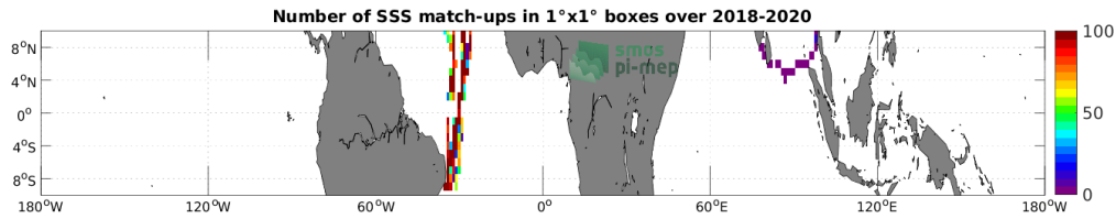
Figure 4: Number of SSS match-ups between TSG (GOSUD-Sailing-ship) SSS and the SMAP SSS L3 v5 - Monthly (RSS) SSS product for the Equatorial Ocean 10N-10S Pi-MEP region over 1^\circ \times 1^\circ boxes and for the full satellite product period.
