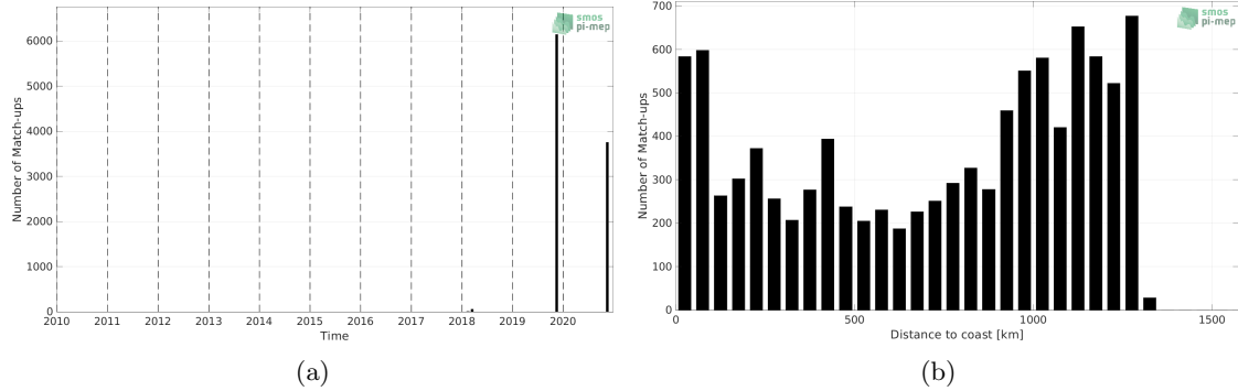
Figure 1: Number of match-ups between TSG (GOSUD-Sailing-ship) and SMAP SSS L3 v5 - Monthly (RSS) SSS as a function of time (a) and as function of the distance to coast (b) over the Equatorial Ocean 10N-10S Pi-MEP region and for the full satellite product period.
