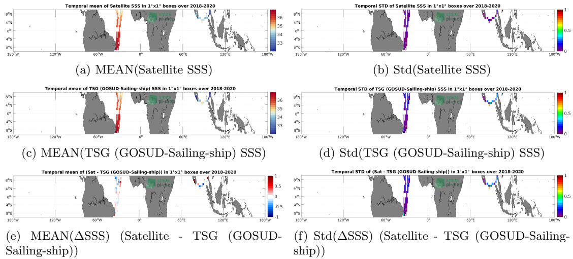
Figure 6: Temporal mean (left) and Std (right) of SSS from SMAP SSS L3 v5 - Monthly (RSS) (top), TSG (GOSUD-Sailing-ship) (middle), and of \Delta SSS (Satellite - TSG (GOSUD-Sailing-ship)). Only match-up pairs are used to generate these maps.
