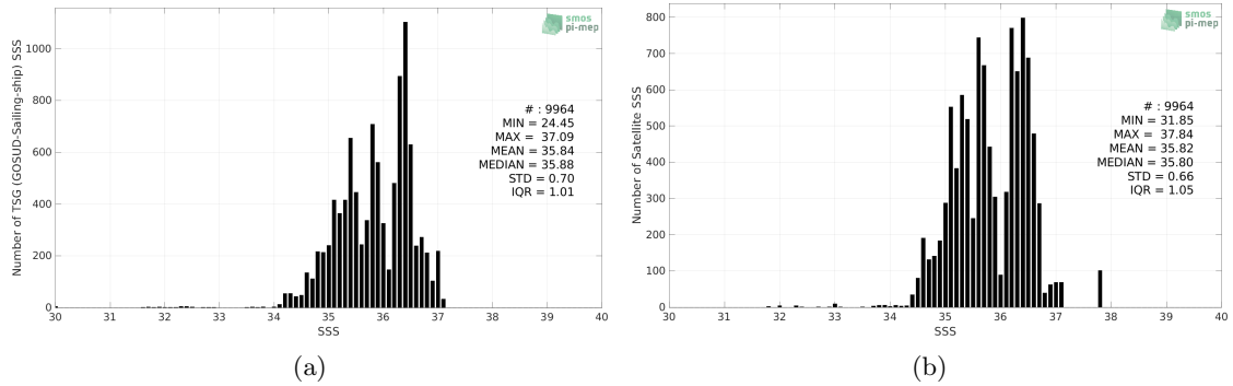
Figure 2: Histograms of SSS from TSG (GOSUD-Sailing-ship) (a) and SMAP SSS L3 v5 - Monthly (RSS) (b) considering all match-up pairs per bins of 0.1 over the Equatorial Ocean 10N-10S Pi-MEP region and for the full satellite product period.
