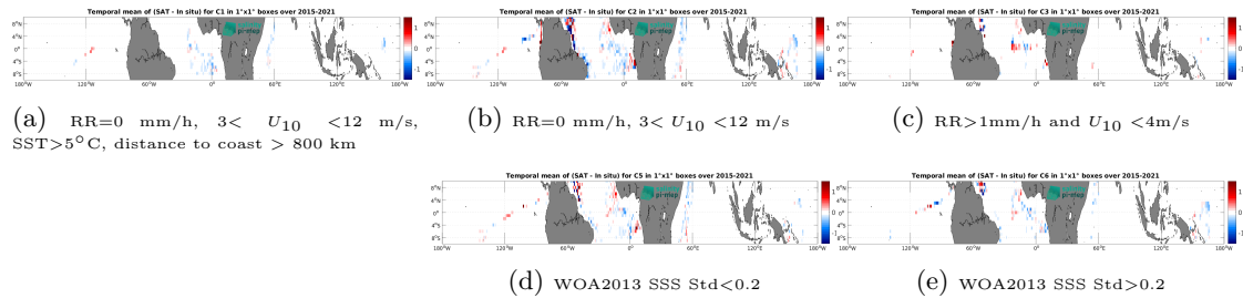
Figure 12: Temporal mean gridded over spatial boxes of size 1^\circ \times 1^\circ of \Delta\text{SSS} (SMAP SSS L3 v5 - Monthly (RSS) - TSG (GOSUD-Research-vessel)) for 5 different subdatasets corresponding to: RR=0 mm/h, 3 < U_{10} < 12 m/s, SST>5°C, distance to coast > 800 km (a), RR=0 mm/h, 3 < U_{10} < 12 m/s (b), RR>1mm/h and U_{10} < 4 m/s (c), WOA2013 SSS Std<0.2 (d), WOA2013 SSS Std>0.2 (e).
