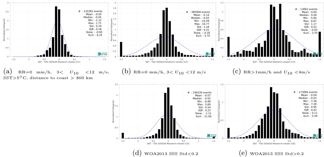
Figure 13: Normalized histogram of \Delta\text{SSS} (SMAP SSS L3 v5 - Monthly (RSS) - TSG (GOSUD-Research-vessel)) for 5 different subdatasets corresponding to: RR=0 mm/h, 3 < U_{10} < 12 m/s, SST>5°C, distance to coast > 800 km (a), RR=0 mm/h, 3 < U_{10} < 12 m/s (b), RR>1mm/h and U_{10} < 4 m/s (c), WOA2013 SSS Std<0.2 (d), WOA2013 SSS Std>0.2 (e).
