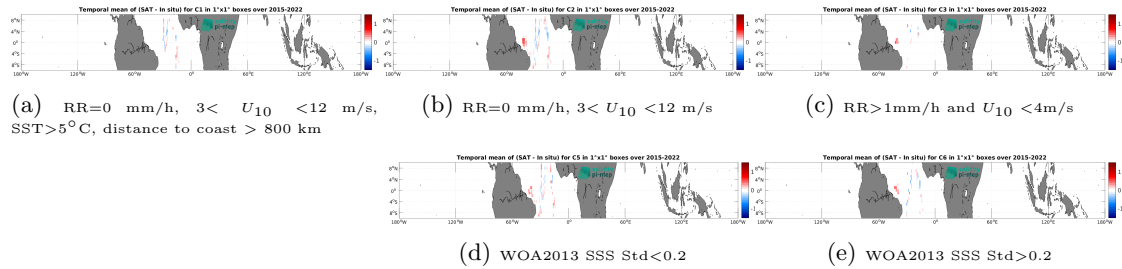
Figure 12: Temporal mean gridded over spatial boxes of size 1^\circ \times 1^\circ of \Delta\text{SSS} (SMAP SSS L3 v5 - Monthly (RSS) - TSG (CSIC-UTM)) for 5 different subdatasets corresponding to:RR=0 mm/h, 3 < U_{10} < 12 m/s, SST >5^\circ\text{C} , distance to coast > 800 km (a), RR=0 mm/h, 3 < U_{10} < 12 m/s (b), RR >1 mm/h and U_{10} < 4 m/s (c), WOA2013 SSS Std <0.2 (d), WOA2013 SSS Std >0.2 (e).
