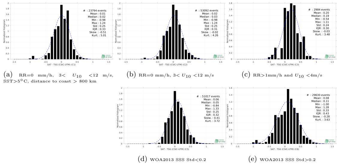
Figure 13: Normalized histogram of \Delta SSS (SMAP SSS L3 v5 - Monthly (RSS) - TSG (CSIC-UTM)) for 5 different subdatasets corresponding to: RR=0 mm/h, 3 < U_{10} < 12 m/s, SST >5^\circ C, distance to coast > 800 km (a), RR=0 mm/h, 3 < U_{10} < 12 m/s (b), RR >1 mm/h and U_{10} < 4 m/s (c), WOA2013 SSS Std <0.2 (d), WOA2013 SSS Std >0.2 (e).
