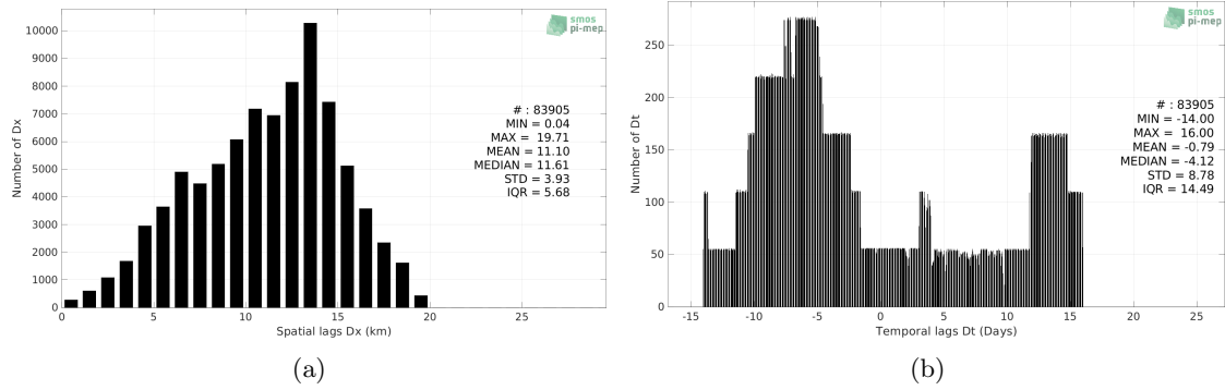
Figure 5: Histograms of the spatial (a) and temporal (b) lags between the location/time of the TSG (CSIC-UTM) measurement and the date of the corresponding SMAP SSS L3 v5 - Monthly (RSS) SSS pixel.
