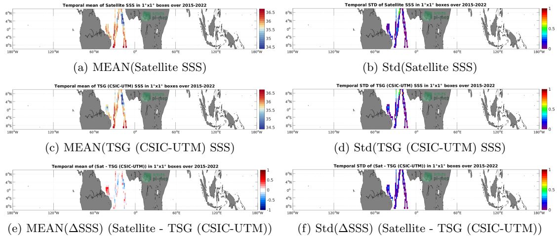
Figure 6: Temporal mean (left) and Std (right) of SSS from SMAP SSS L3 v5 - Monthly (RSS) (top), TSG (CSIC-UTM) (middle), and of \Delta SSS (Satellite - TSG (CSIC-UTM)). Only match-up pairs are used to generate these maps.
