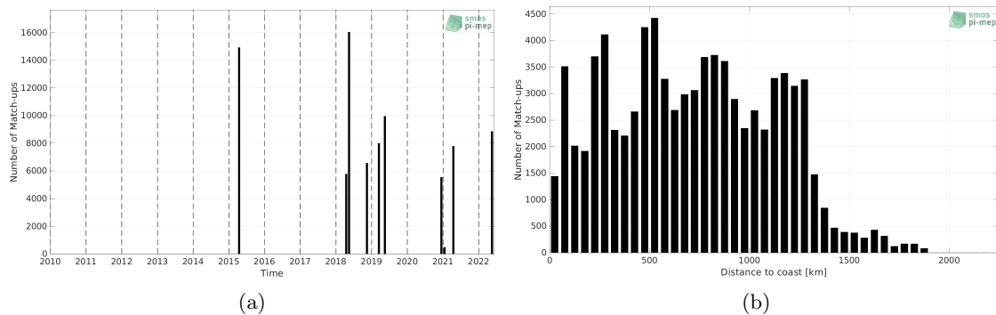
Figure 1: Number of match-ups between TSG (CSIC-UTM) and SMAP SSS L3 v5 - Monthly (RSS) SSS as a function of time (a) and as function of the distance to coast (b) over the Equatorial Ocean 10N-10S Pi-MEP region and for the full satellite product period.
