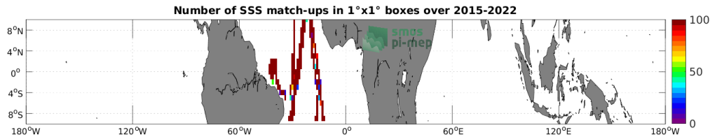
Figure 4: Number of SSS match-ups between TSG (CSIC-UTM) SSS and the SMAP SSS L3 v5 - Monthly (RSS) SSS product for the Equatorial Ocean 10N-10S Pi-MEP region over 1^\circ \times 1^\circ boxes and for the full satellite product period.
