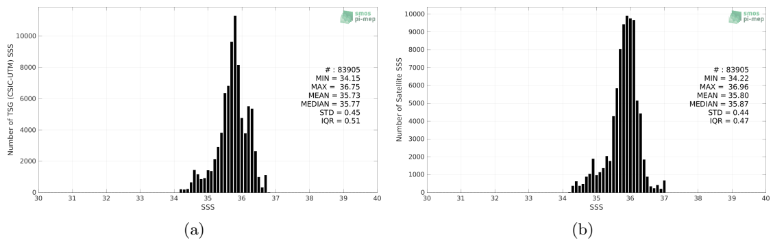
Figure 2: Histograms of SSS from TSG (CSIC-UTM) (a) and SMAP SSS L3 v5 - Monthly (RSS) (b) considering all match-up pairs per bins of 0.1 over the Equatorial Ocean 10N-10S Pi-MEP region and for the full satellite product period.
