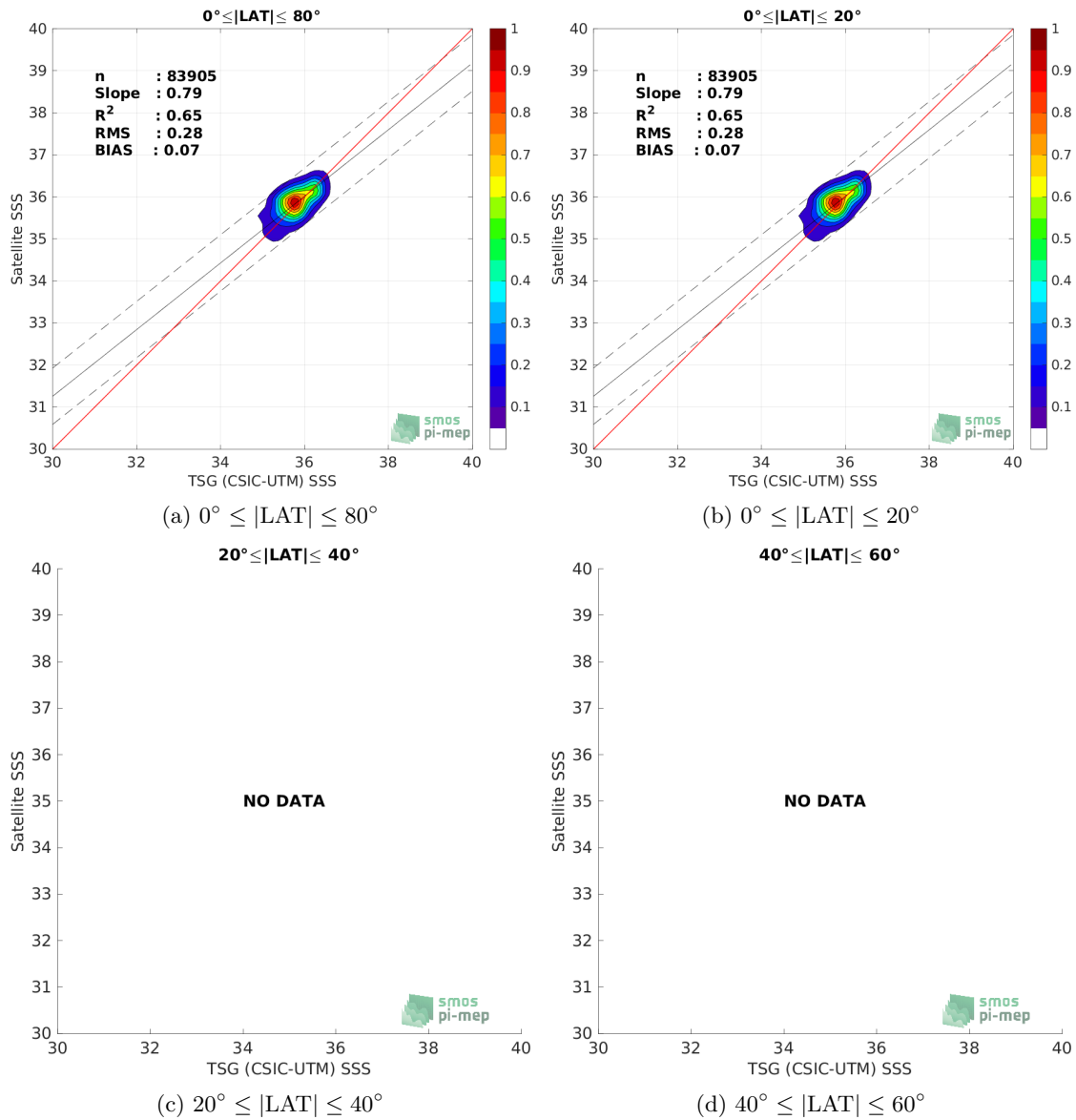
Figure 9: Contour maps of the concentration of SMAP SSS L3 v5 - Monthly (RSS) SSS (y-axis) versus TSG (CSIC-UTM) SSS (x-axis) at match-up pairs for different latitude bands. For each plot, the red line shows x=y . The black thin and dashed lines indicate a linear fit through the data cloud and the \pm 95\% confidence levels, respectively. The number match-up pairs n , the slope and R^2 coefficient of the linear fit, the root mean square (RMS) and the mean bias between satellite and in situ data are indicated for each latitude band in each plots.
