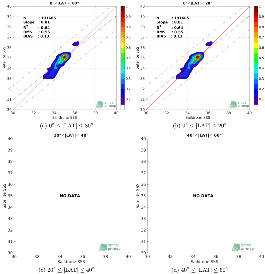
Figure 9: Contour maps of the concentration of SMAP SSS L3 v5 - Monthly (RSS) SSS (y-axis) versus Saildrone SSS (x-axis) at match-up pairs for different latitude bands. For each plot, the red line shows x=y . The black thin and dashed lines indicate a linear fit through the data cloud and the \pm 95\% confidence levels, respectively. The number match-up pairs n , the slope and R^2 coefficient of the linear fit, the root mean square (RMS) and the mean bias between satellite and in situ data are indicated for each latitude band in each plots.
