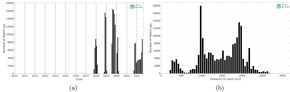
Figure 1: Number of match-ups between Saildrone and SMAP SSS L3 v5 - Monthly (RSS) SSS as a function of time (a) and as function of the distance to coast (b) over the Equatorial Ocean 10N-10S Pi-MEP region and for the full satellite product period.
