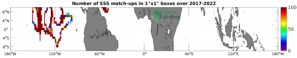
Figure 4: Number of SSS match-ups between Saildrone SSS and the SMAP SSS L3 v5 - Monthly (RSS) SSS product for the Equatorial Ocean 10N-10S Pi-MEP region over 1^\circ \times 1^\circ boxes and for the full satellite product period.
