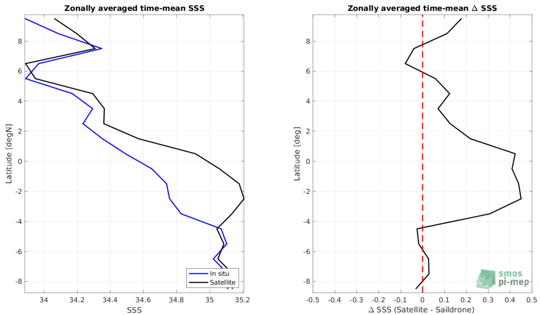
Figure 8: Left panel: Zonal mean SSS from SMAP SSS L3 v5 - Monthly (RSS) satellite product (black) and from Sairdron (blue). Right panel: Zonal mean of \Delta SSS (Satellite - Sairdron) for all the collected Pi-MEP match-up pairs estimated over the full satellite product period.
