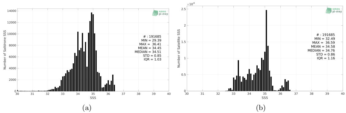
Figure 2: Histograms of SSS from Saildrone (a) and SMAP SSS L3 v5 - Monthly (RSS) (b) considering all match-up pairs per bins of 0.1 over the Equatorial Ocean 10N-10S Pi-MEP region and for the full satellite product period.
