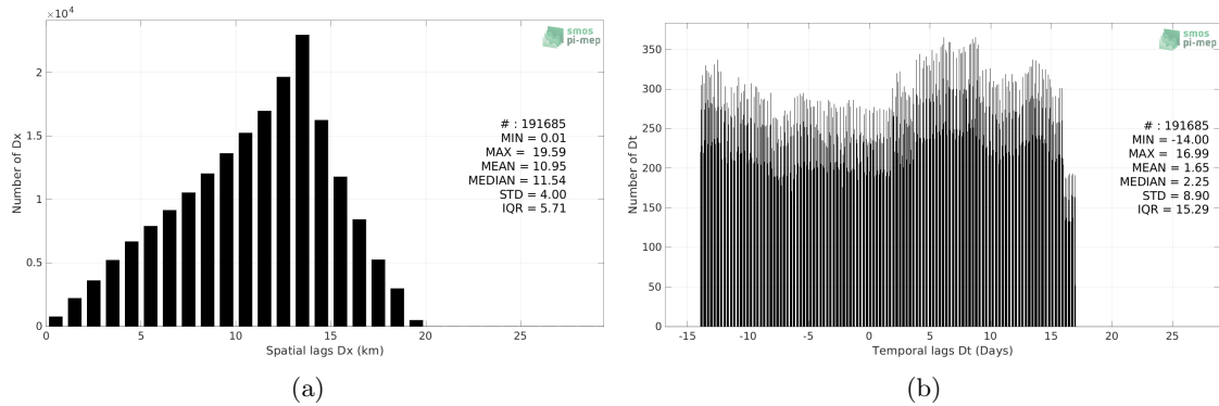
Figure 5: Histograms of the spatial (a) and temporal (b) lags between the location/time of the Saildrone measurement and the date of the corresponding SMAP SSS L3 v5 - Monthly (RSS) SSS pixel.
