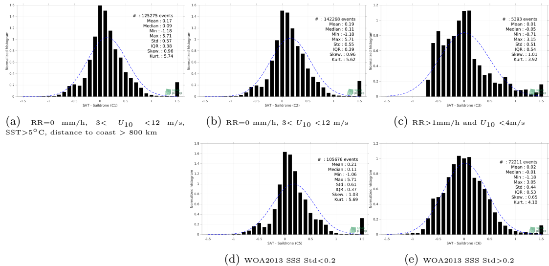
Figure 13: Normalized histogram of \Delta SSS (SMAP SSS L3 v5 - Monthly (RSS) - Saildrone) for 5 different subdatasets corresponding to: RR=0 mm/h, 3 < U_{10} < 12 m/s, SST > 5^\circ C , distance to coast > 800 km (a), RR=0 mm/h, 3 < U_{10} < 12 m/s (b), RR>1mm/h and U_{10} < 4 m/s (c), WOA2013 SSS Std<0.2 (d), WOA2013 SSS Std>0.2 (e).
