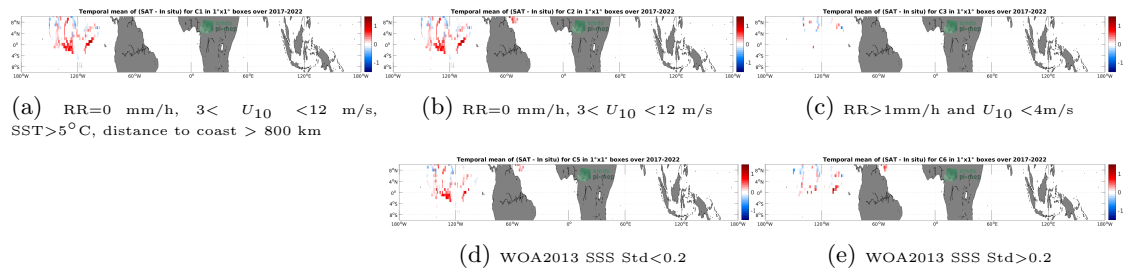
Figure 12: Temporal mean gridded over spatial boxes of size 1^\circ \times 1^\circ of \Delta SSS (SMAP SSS L3 v5 - Monthly (RSS) - Saildrone) for 5 different subdatasets corresponding to:RR=0 mm/h, 3 < U_{10} < 12 m/s, SST > 5^\circ C , distance to coast > 800 km (a), RR=0 mm/h, 3 < U_{10} < 12 m/s (b), RR>1mm/h and U_{10} < 4 m/s (c), WOA2013 SSS Std<0.2 (d), WOA2013 SSS Std>0.2 (e).
