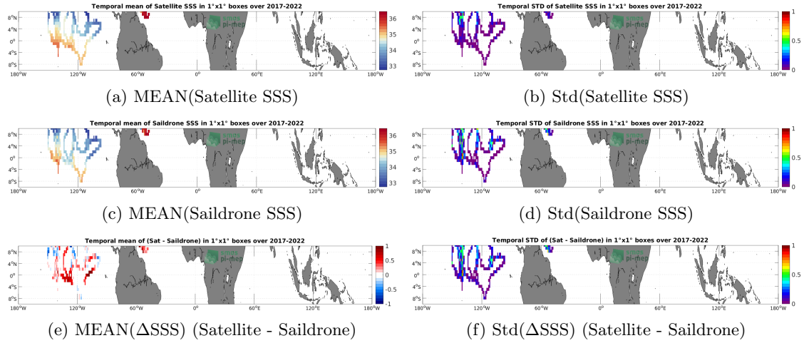
Figure 6: Temporal mean (left) and Std (right) of SSS from SMAP SSS L3 v5 - Monthly (RSS) (top), Saildrone (middle), and of \Delta SSS (Satellite - Saildrone). Only match-up pairs are used to generate these maps.
