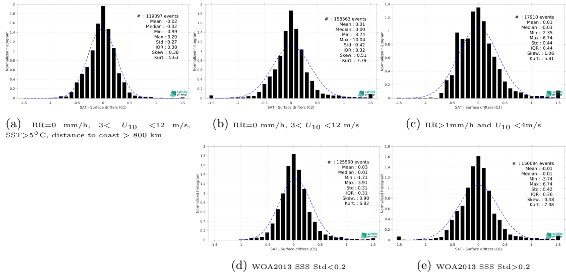
Figure 12: Normalized histogram of \Delta SSS (SMAP SSS L3 v5 - Monthly (RSS) - Surface drifters) for 5 different subdatasets corresponding to: RR=0 mm/h, 3 < U_{10} < 12 m/s, SST >5^\circ\text{C} , distance to coast > 800 km (a), RR=0 mm/h, 3 < U_{10} < 12 m/s (b), RR >1 mm/h and U_{10} < 4 m/s (c), WOA2013 SSS Std <0.2 (d), WOA2013 SSS Std >0.2 (e).
