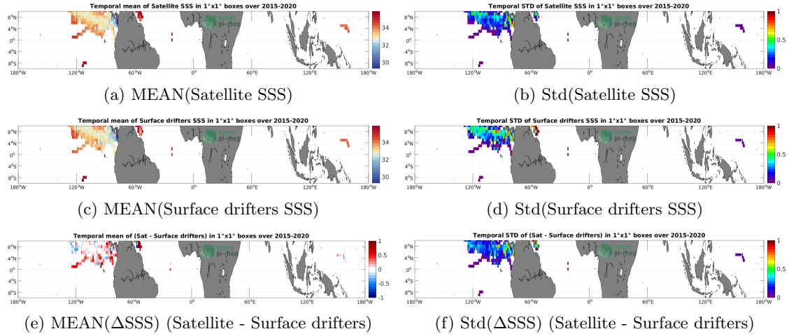
Figure 5: Temporal mean (left) and Std (right) of SSS from SMAP SSS L3 v5 - Monthly (RSS) (top), Surface drifters (middle), and of \Delta SSS (Satellite - Surface drifters). Only match-up pairs are used to generate these maps.
