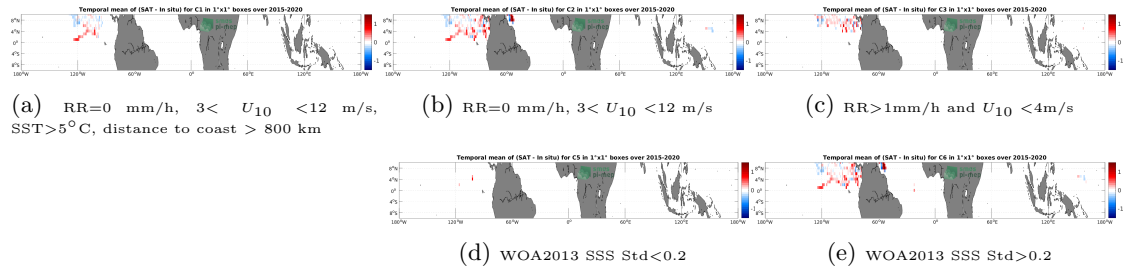
Figure 11: Temporal mean gridded over spatial boxes of size 1^\circ \times 1^\circ of \Delta SSS (SMAP SSS L3 v5 - Monthly (RSS) - Surface drifters) for 5 different subdatasets corresponding to:RR=0 mm/h, 3 < U_{10} < 12 m/s, SST > 5^\circ C , distance to coast > 800 km (a), RR=0 mm/h, 3 < U_{10} < 12 m/s (b), RR>1mm/h and U_{10} < 4 m/s (c), WOA2013 SSS Std<0.2 (d), WOA2013 SSS Std>0.2 (e).
