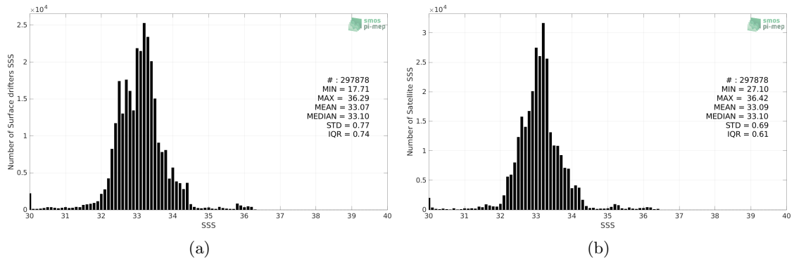
Figure 2: Histograms of SSS from Surface drifters (a) and SMAP SSS L3 v5 - Monthly (RSS) (b) considering all match-up pairs per bins of 0.1 over the Equatorial Ocean 10N-10S Pi-MEP region and for the full satellite product period.
