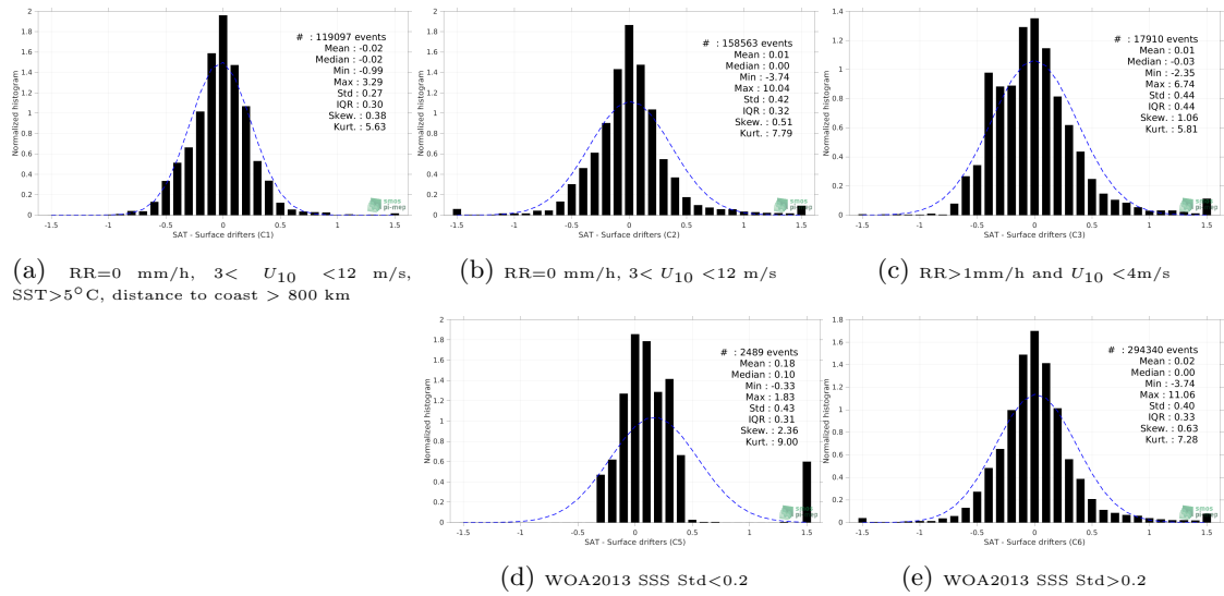
Figure 12: Normalized histogram of \Delta SSS (SMAP SSS L3 v5 - Monthly (RSS) - Surface drifters) for 5 different subdatasets corresponding to: RR=0 mm/h, 3 < U_{10} < 12 m/s, SST > 5^\circ C , distance to coast > 800 km (a), RR=0 mm/h, 3 < U_{10} < 12 m/s (b), RR>1mm/h and U_{10} < 4 m/s (c), WOA2013 SSS Std<0.2 (d), WOA2013 SSS Std>0.2 (e).
