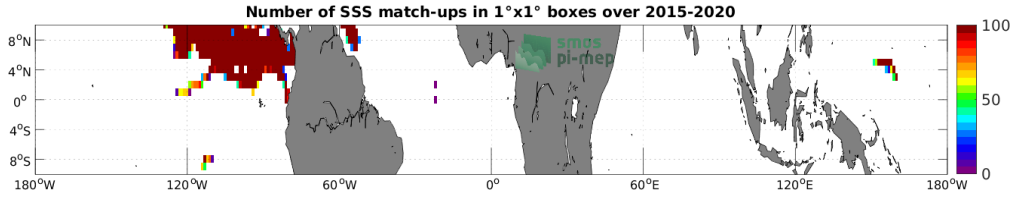
Figure 3: Number of SSS match-ups between Surface drifters SSS and the SMAP SSS L3 v5 - Monthly (RSS) SSS product for the Equatorial Ocean 10N-10S Pi-MEP region over 1^\circ \times 1^\circ boxes and for the full satellite product period.
