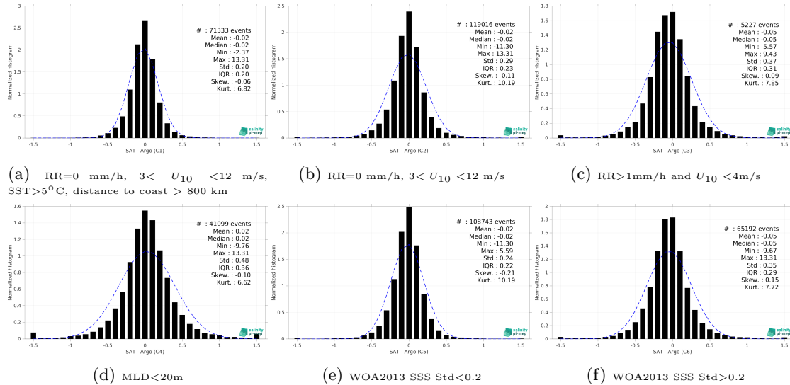
Figure 13: Normalized histogram of \Delta SSS (SMAP SSS L3 v5 - Monthly (RSS) - Argo) for 6 different subdatasets corresponding to: RR=0 mm/h, 3 < U_{10} < 12 m/s, SST >5^\circ C, distance to coast > 800 km (a), RR=0 mm/h, 3 < U_{10} < 12 m/s (b), RR >1 mm/h and U_{10} < 4 m/s (c), MLD <20 m (d), WOA2013 SSS Std <0.2 (e), WOA2013 SSS Std >0.2 (f).
