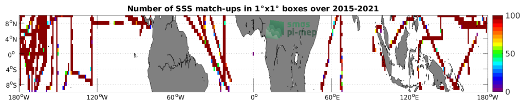
Figure 4: Number of SSS match-ups between TSG (SAMOS) SSS and the SMAP SSS L3 v4 - 8-Day running (RSS) SSS product for the Equatorial Ocean 10N-10S Pi-MEP region over 1^\circ \times 1^\circ boxes and for the full satellite product period.
