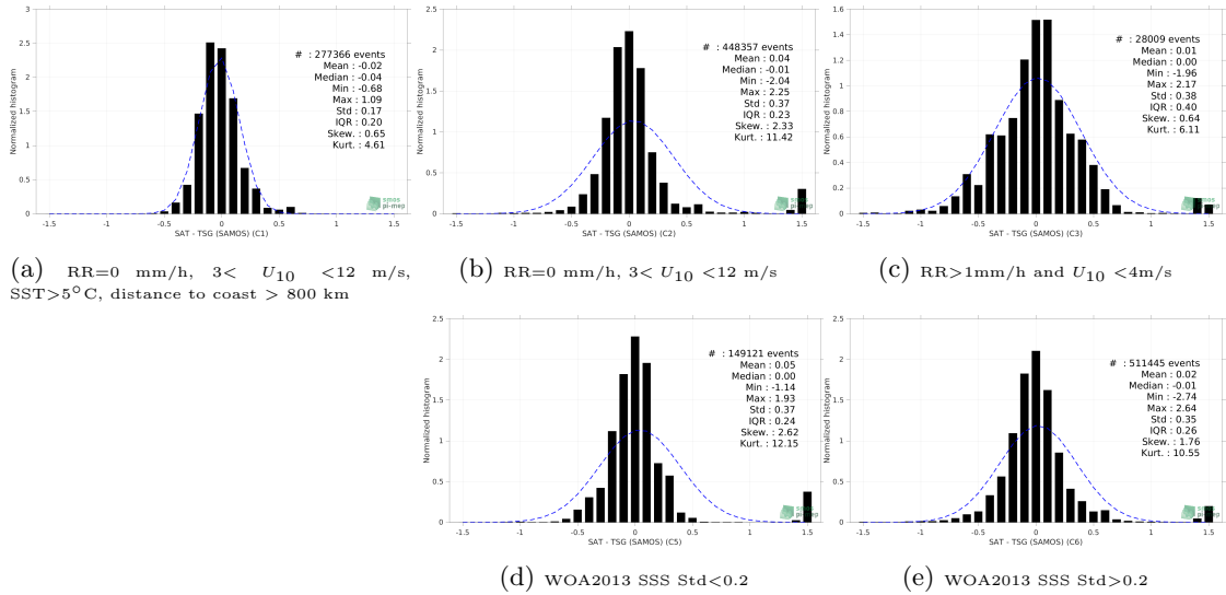
Figure 13: Normalized histogram of \Delta SSS (SMAP SSS L3 v4 - 8-Day running (RSS) - TSG (SAMOS)) for 5 different subdatasets corresponding to: RR=0 mm/h, 3 < U_{10} < 12 m/s, SST >5^\circ C, distance to coast > 800 km (a), RR=0 mm/h, 3 < U_{10} < 12 m/s (b), RR >1 mm/h and U_{10} < 4 m/s (c), WOA2013 SSS Std <0.2 (d), WOA2013 SSS Std >0.2 (e).
