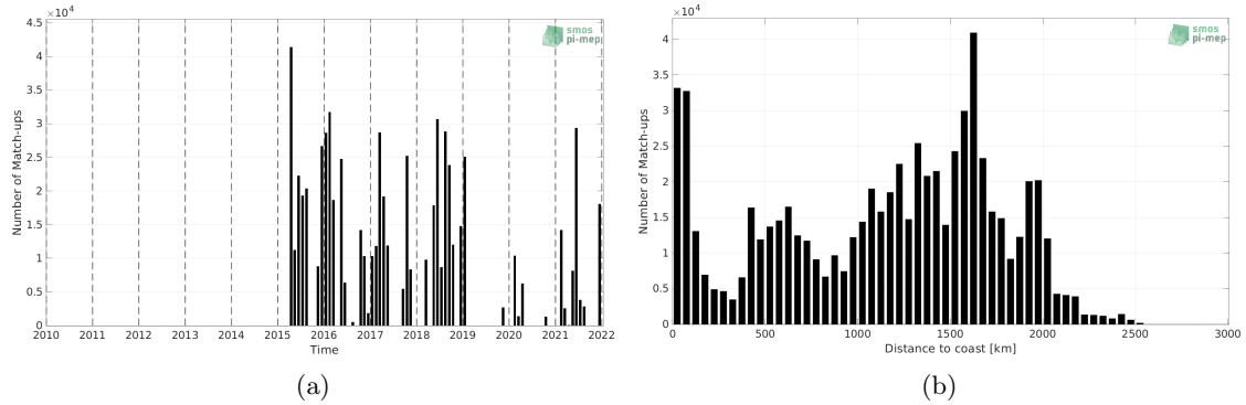
Figure 1: Number of match-ups between TSG (SAMOS) and SMAP SSS L3 v4 - 8-Day running (RSS) SSS as a function of time (a) and as function of the distance to coast (b) over the Equatorial Ocean 10N-10S Pi-MEP region and for the full satellite product period.
