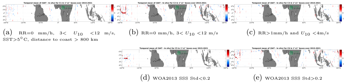
Figure 12: Temporal mean gridded over spatial boxes of size 1^\circ \times 1^\circ of \Delta SSS (SMAP SSS L3 v4 - 8-Day running (RSS) - TSG (SAMOS)) for 5 different subdatasets corresponding to:RR=0 mm/h, 3 < U_{10} < 12 m/s, SST >5^\circ C, distance to coast > 800 km (a), RR=0 mm/h, 3 < U_{10} < 12 m/s (b), RR >1 mm/h and U_{10} < 4 m/s (c), WOA2013 SSS Std <0.2 (d), WOA2013 SSS Std >0.2 (e).
