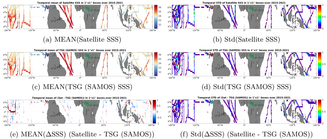
Figure 6: Temporal mean (left) and Std (right) of SSS from SMAP SSS L3 v4 - 8-Day running (RSS) (top), TSG (SAMOS) (middle), and of \Delta SSS (Satellite - TSG (SAMOS)). Only match-up pairs are used to generate these maps.
