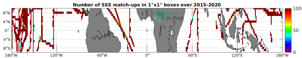
Figure 4: Number of SSS match-ups between TSG (SAMOS) SSS and the SMAP SSS L3 v4 - 8-Day running (RSS) SSS product for the Equatorial Ocean 10N-10S Pi-MEP region over 1°x1° boxes and for the full satellite product period.
