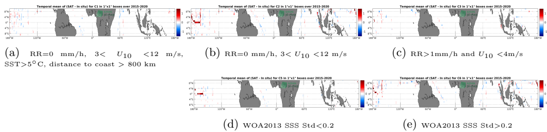
Figure 12: Temporal mean gridded over spatial boxes of size 1°x1° of \Delta SSS (SMAP SSS L3 v4 - 8-Day running (RSS) - TSG (SAMOS)) for 5 different subdatasets corresponding to:RR=0 mm/h, 3 < U_{10} < 12 m/s, SST>5°C, distance to coast > 800 km (a), RR=0 mm/h, 3 < U_{10} < 12 m/s (b), RR>1mm/h and U_{10} < 4m/s (c), WOA2013 SSS Std<0.2 (d), WOA2013 SSS Std>0.2 (e).
