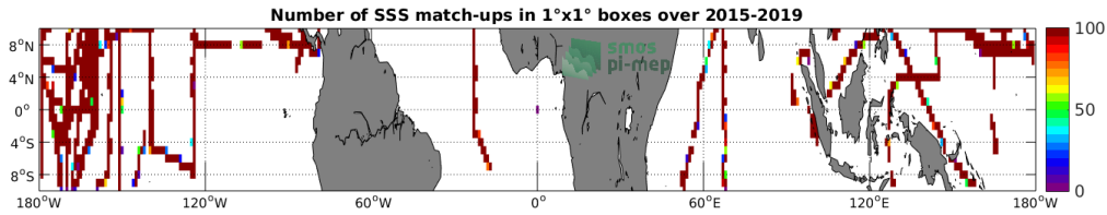
Figure 4: Number of SSS match-ups between TSG-SAMOS SSS and the SMAP-L3-RSS-V4-8DAY-RUNNING SSS product for the Equatorial Ocean 10N-10S Pi-MEP region over 1°x1° boxes and for the full satellite product period.
