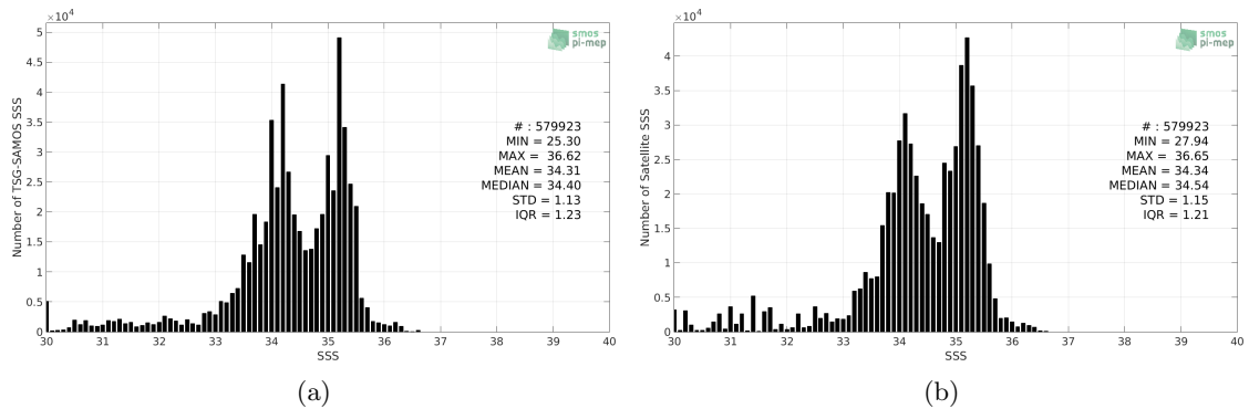
Figure 2: Histograms of SSS from TSG-SAMOS (a) and SMAP-L3-RSS-V4-8DAY-RUNNING (b) considering all match-up pairs per bins of 0.1 over the Equatorial Ocean 10N-10S Pi-MEP region and for the full satellite product period.
