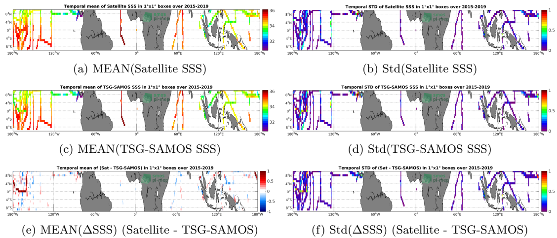
Figure 6: Temporal mean (left) and Std (right) of SSS from SMAP-L3-RSS-V4-8DAY-RUNNING (top), TSG-SAMOS (middle), and of \Delta SSS (Satellite - TSG-SAMOS). Only match-up pairs are used to generate these maps.
