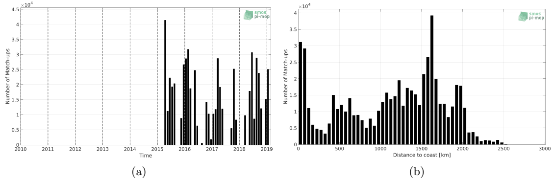
Figure 1: Number of match-ups between TSG-SAMOS and SMAP-L3-RSS-V4-8DAY-RUNNING SSS as a function of time (a) and as function of the distance to coast (b) over the Equatorial Ocean 10N-10S Pi-MEP region and for the full satellite product period.
