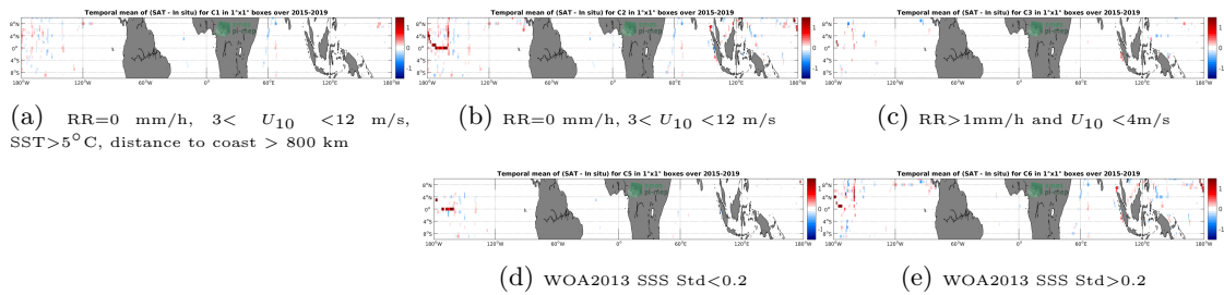
Figure 12: Temporal mean gridded over spatial boxes of size 1°x1° of \Delta SSS (SMAP-L3-RSS-V4-8DAY-RUNNING - TSG-SAMOS) for 5 different subdatasets corresponding to:RR=0 mm/h, 3 < U_{10} < 12 m/s, SST > 5°C, distance to coast > 800 km (a), RR=0 mm/h, 3 < U_{10} < 12 m/s (b), RR > 1mm/h and U_{10} < 4m/s (c), WOA2013 SSS Std < 0.2 (d), WOA2013 SSS Std > 0.2 (e).
