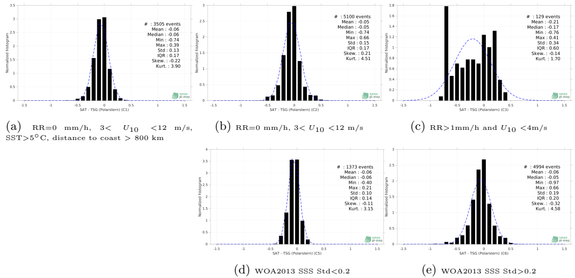
Figure 13: Normalized histogram of \Delta SSS (SMAP SSS L3 v4 - 8-Day running (RSS) - TSG (Polarstern)) for 5 different subdatasets corresponding to: RR=0 mm/h, 3 < U_{10} < 12 m/s, SST >5^\circ\text{C} , distance to coast > 800 km (a), RR=0 mm/h, 3 < U_{10} < 12 m/s (b), RR >1 mm/h and U_{10} < 4 m/s (c), WOA2013 SSS Std <0.2 (d), WOA2013 SSS Std >0.2 (e).
