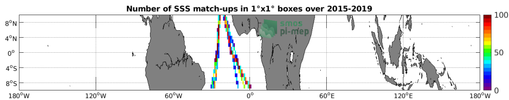
Figure 4: Number of SSS match-ups between TSG (Polarstern) SSS and the SMAP SSS L3 v4 - 8-Day running (RSS) SSS product for the Equatorial Ocean 10N-10S Pi-MEP region over 1^\circ \times 1^\circ boxes and for the full satellite product period.
