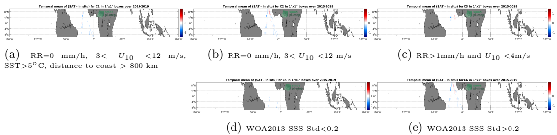
Figure 12: Temporal mean gridded over spatial boxes of size 1°x1° of ΔSSS (SMAP SSS L3 v4 - 8-Day running (RSS) - TSG (Polarstern)) for 5 different subdatasets corresponding to:RR=0 mm/h, 3 < U 10 < 12 m/s, SST>5°C, distance to coast > 800 km (a), RR=0 mm/h, 3 < U 10 < 12 m/s (b), RR>1mm/h and U 10 < 4m/s (c), WOA2013 SSS Std<0.2 (d), WOA2013 SSS Std>0.2 (e).
