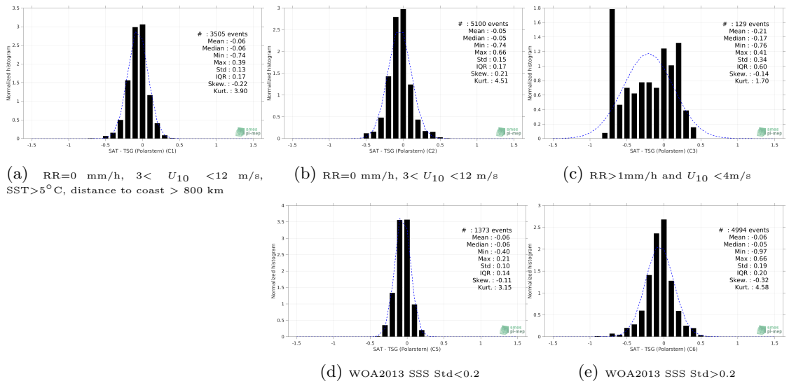
Figure 13: Normalized histogram of ΔSSS (SMAP SSS L3 v4 - 8-Day running (RSS) - TSG (Polarstern)) for 5 different subdatasets corresponding to: RR=0 mm/h, 3 < U 10 < 12 m/s, SST>5°C, distance to coast > 800 km (a), RR=0 mm/h, 3 < U 10 < 12 m/s (b), RR>1mm/h and U 10 < 4m/s (c), WOA2013 SSS Std<0.2 (d), WOA2013 SSS Std>0.2 (e).
