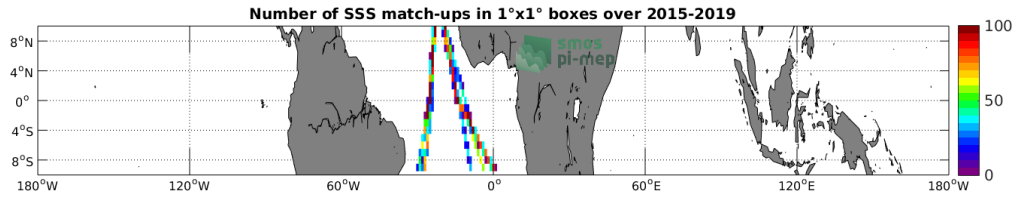
Figure 4: Number of SSS match-ups between TSG-POLARSTERN SSS and the SMAP-L3-RSS-V4-8DAY-RUNNING SSS product for the Equatorial Ocean 10N-10S Pi-MEP region over 1^\circ \times 1^\circ boxes and for the full satellite product period.
