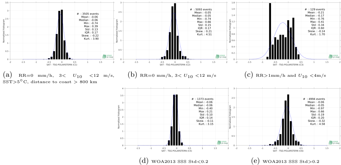
Figure 13: Normalized histogram of ΔSSS (SMAP-L3-RSS-V4-8DAY-RUNNING - TSG-POLARSTERN) for 5 different subdatasets corresponding to: RR=0 mm/h, 3 < U 10 < 12 m/s, SST > 5°C, distance to coast > 800 km (a), RR=0 mm/h, 3 < U 10 < 12 m/s (b), RR > 1mm/h and U 10 < 4m/s (c), WOA2013 SSS Std < 0.2 (d), WOA2013 SSS Std > 0.2 (e).
