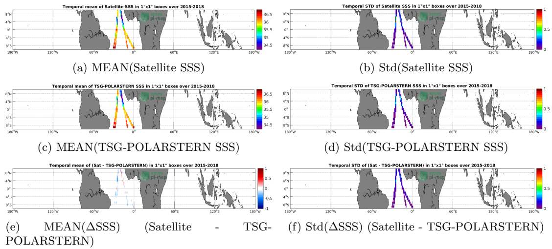
Figure 6: Temporal mean (left) and Std (right) of SSS from SMAP-L3-RSS-V4-8DAY-RUNNING (top), TSG-POLARSTERN (middle), and of \Delta SSS (Satellite - TSG-POLARSTERN). Only match-up pairs are used to generate these maps.
