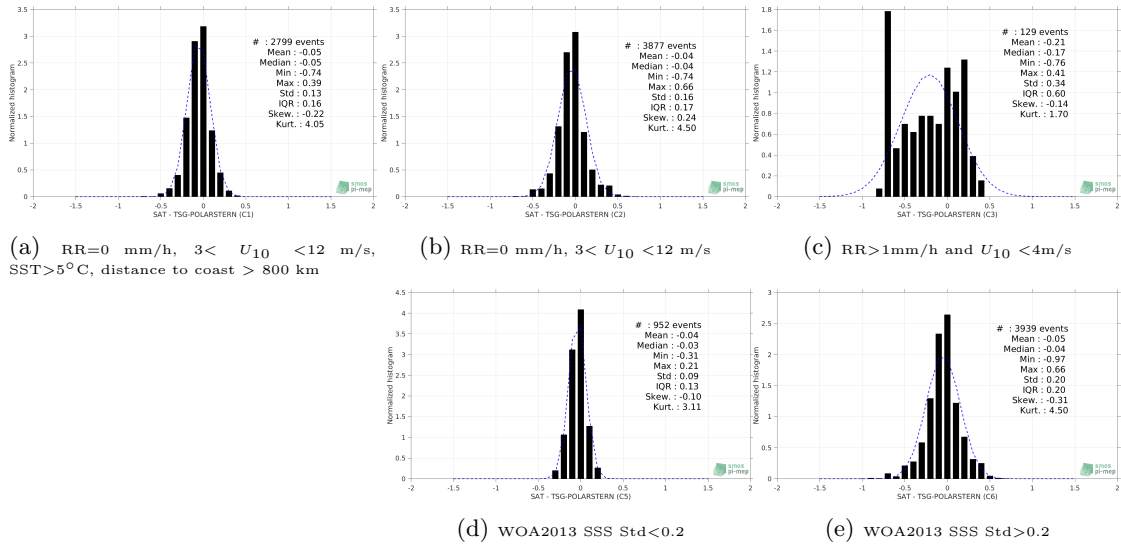
Figure 13: Normalized histogram of ΔSSS (SMAP-L3-RSS-V4-8DAY-RUNNING - TSG-POLARSTERN) for 5 different subdatasets corresponding to: RR=0 mm/h, 3 < U 10 < 12 m/s, SST>5°C, distance to coast > 800 km (a), RR=0 mm/h, 3 < U 10 < 12 m/s (b), RR>1mm/h and U 10 < 4m/s (c), WOA2013 SSS Std<0.2 (d), WOA2013 SSS Std>0.2 (e).
