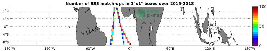
Figure 4: Number of SSS match-ups between TSG-POLARSTERN SSS and the SMAP-L3-RSS-V4-8DAY-RUNNING SSS product for the Equatorial Ocean 10N-10S Pi-MEP region over 1°x1° boxes and for the full satellite product period.
