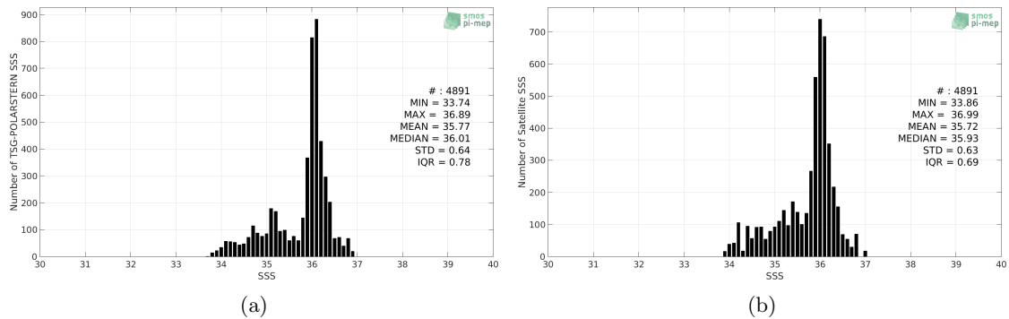
Figure 2: Histograms of SSS from TSG-POLARSTERN (a) and SMAP-L3-RSS-V4-8DAY-RUNNING (b) considering all match-up pairs per bins of 0.1 over the Equatorial Ocean 10N-10S Pi-MEP region and for the full satellite product period.
