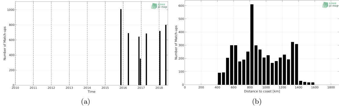
Figure 1: Number of match-ups between TSG-POLARSTERN and SMAP-L3-RSS-V4-8DAY-RUNNING SSS as a function of time (a) and as function of the distance to coast (b) over the Equatorial Ocean 10N-10S Pi-MEP region and for the full satellite product period.
