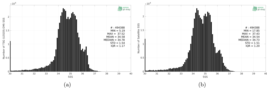
Figure 2: Histograms of SSS from TSG (LEGOS-DM) (a) and SMAP SSS L3 v4 - 8-Day running (RSS) (b) considering all match-up pairs per bins of 0.1 over the Equatorial Ocean 10N-10S Pi-MEP region and for the full satellite product period.
