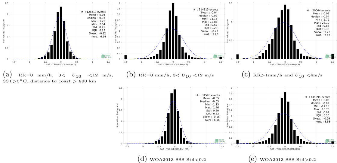
Figure 13: Normalized histogram of \Delta SSS (SMAP SSS L3 v4 - 8-Day running (RSS) - TSG (LEGOS-DM)) for 5 different subdatasets corresponding to: RR=0 mm/h, 3 < U_{10} < 12 m/s, SST > 5^\circ C , distance to coast > 800 km (a), RR=0 mm/h, 3 < U_{10} < 12 m/s (b), RR>1mm/h and U_{10} < 4m/s (c), WOA2013 SSS Std<0.2 (d), WOA2013 SSS Std>0.2 (e).
