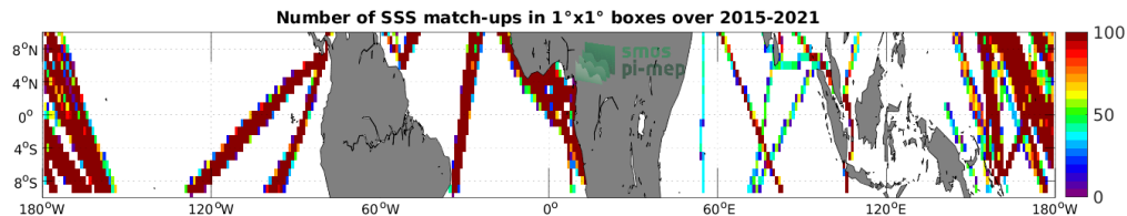
Figure 4: Number of SSS match-ups between TSG (LEGOS-DM) SSS and the SMAP SSS L3 v4 - 8-Day running (RSS) SSS product for the Equatorial Ocean 10N-10S Pi-MEP region over 1^\circ \times 1^\circ boxes and for the full satellite product period.
