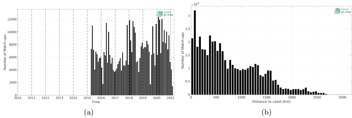
Figure 1: Number of match-ups between TSG (LEGOS-DM) and SMAP SSS L3 v4 - 8-Day running (RSS) SSS as a function of time (a) and as function of the distance to coast (b) over the Equatorial Ocean 10N-10S Pi-MEP region and for the full satellite product period.
