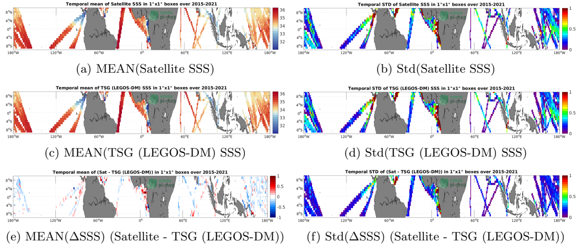
Figure 6: Temporal mean (left) and Std (right) of SSS from SMAP SSS L3 v4 - 8-Day running (RSS) (top), TSG (LEGOS-DM) (middle), and of \Delta SSS (Satellite - TSG (LEGOS-DM)). Only match-up pairs are used to generate these maps.
