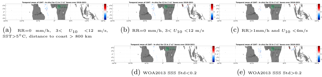
Figure 12: Temporal mean gridded over spatial boxes of size 1^\circ \times 1^\circ of \Delta SSS (SMAP SSS L3 v4 - 8-Day running (RSS) - TSG (GOSUD-Sailing-ship)) for 5 different subdatasets corresponding to: RR=0 mm/h, 3 < U_{10} < 12 m/s, SST>5°C, distance to coast > 800 km (a), RR=0 mm/h, 3 < U_{10} < 12 m/s (b), RR>1mm/h and U_{10} < 4 m/s (c), WOA2013 SSS Std<0.2 (d), WOA2013 SSS Std>0.2 (e).
