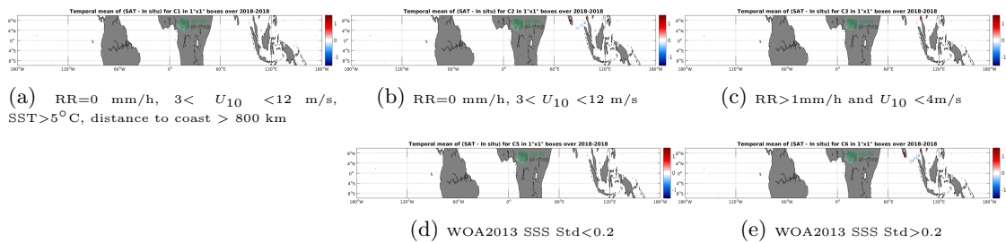
Figure 12: Temporal mean gridded over spatial boxes of size 1^\circ \times 1^\circ of \Delta SSS (SMAP SSS L3 v4 - 8-Day running (RSS) - TSG (GOSUD-Sailing-ship)) for 5 different subdatasets corresponding to: RR=0 mm/h, 3 < U_{10} < 12 m/s, SST>5°C, distance to coast > 800 km (a), RR=0 mm/h, 3 < U_{10} < 12 m/s (b), RR>1mm/h and U_{10} < 4 m/s (c), WOA2013 SSS Std<0.2 (d), WOA2013 SSS Std>0.2 (e).
