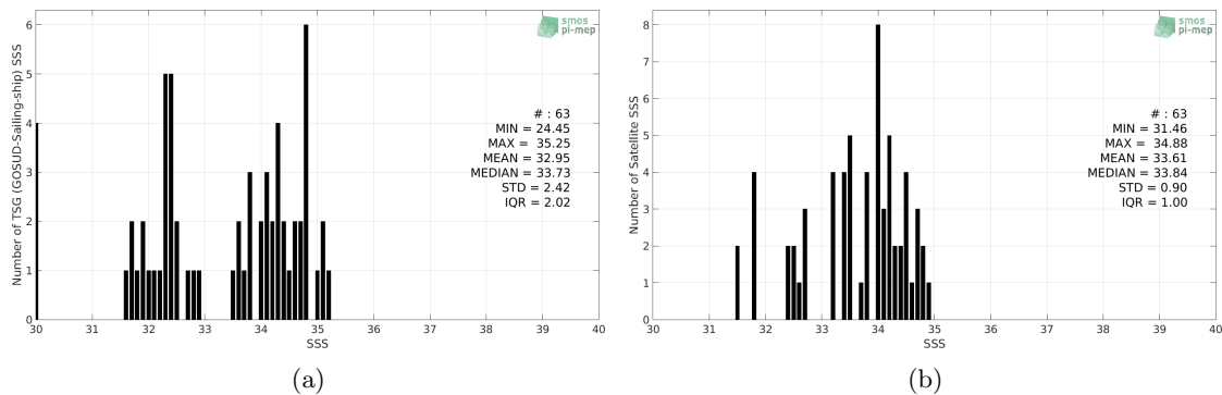
Figure 2: Histograms of SSS from TSG (GOSUD-Sailing-ship) (a) and SMAP SSS L3 v4 - 8-Day running (RSS) (b) considering all match-up pairs per bins of 0.1 over the Equatorial Ocean 10N-10S Pi-MEP region and for the full satellite product period.
