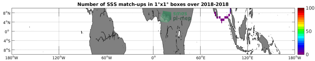
Figure 4: Number of SSS match-ups between TSG (GOSUD-Sailing-ship) SSS and the SMAP SSS L3 v4 - 8-Day running (RSS) SSS product for the Equatorial Ocean 10N-10S Pi-MEP region over 1^\circ \times 1^\circ boxes and for the full satellite product period.
