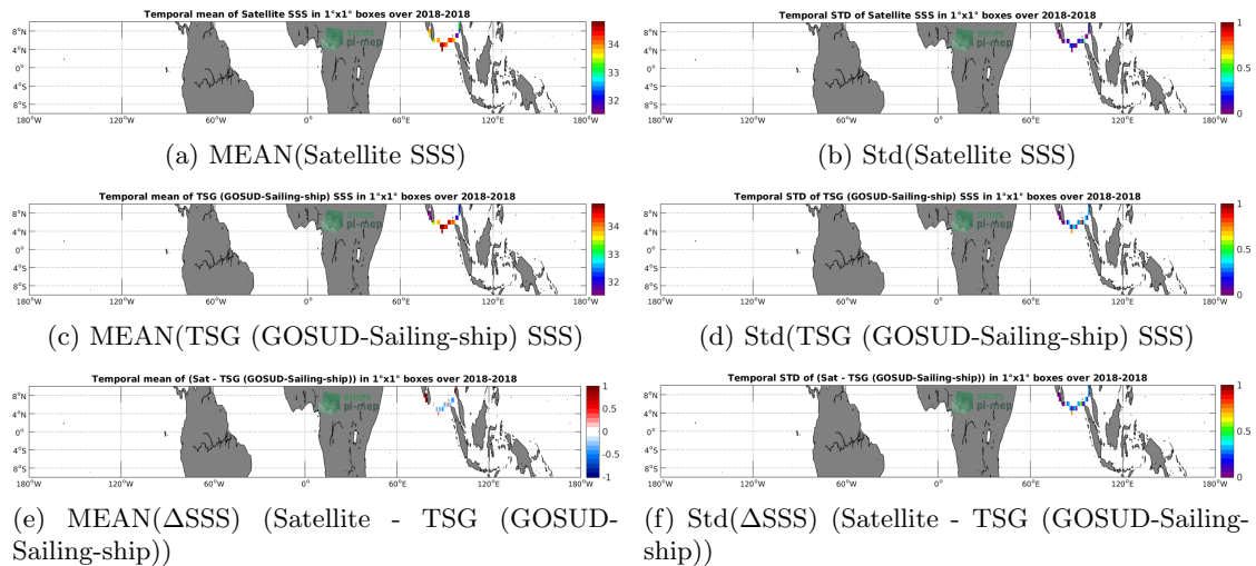
Figure 6: Temporal mean (left) and Std (right) of SSS from SMAP SSS L3 v4 - 8-Day running (RSS) (top), TSG (GOSUD-Sailing-ship) (middle), and of \Delta SSS (Satellite - TSG (GOSUD-Sailing-ship)). Only match-up pairs are used to generate these maps.
