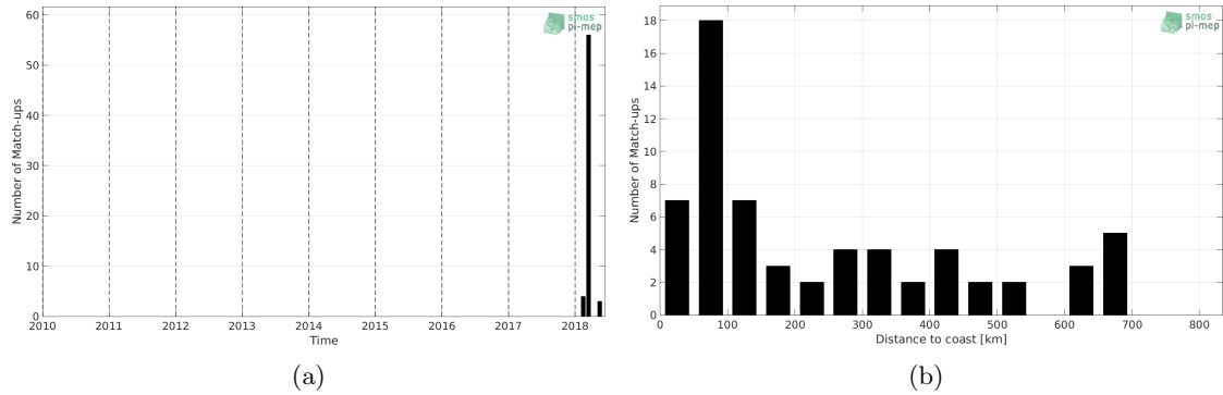
Figure 1: Number of match-ups between TSG (GOSUD-Sailing-ship) and SMAP SSS L3 v4 - 8-Day running (RSS) SSS as a function of time (a) and as function of the distance to coast (b) over the Equatorial Ocean 10N-10S Pi-MEP region and for the full satellite product period.
