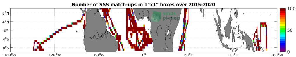
Figure 4: Number of SSS match-ups between TSG (GOSUD-Research-vessel) SSS and the SMAP SSS L3 v4 - 8-Day running (RSS) SSS product for the Equatorial Ocean 10N-10S Pi-MEP region over 1^\circ \times 1^\circ boxes and for the full satellite product period.
