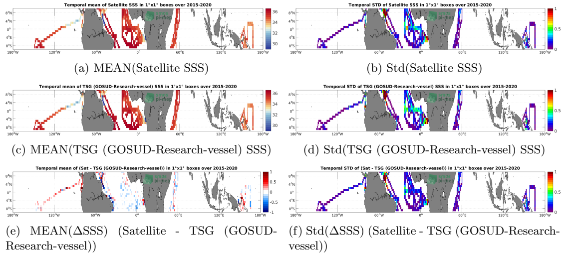
Figure 6: Temporal mean (left) and Std (right) of SSS from SMAP SSS L3 v4 - 8-Day running (RSS) (top), TSG (GOSUD-Research-vessel) (middle), and of \Delta SSS (Satellite - TSG (GOSUD-Research-vessel)). Only match-up pairs are used to generate these maps.
