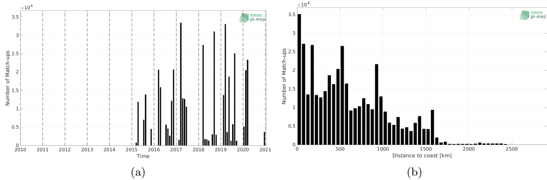
Figure 1: Number of match-ups between TSG (GOSUD-Research-vessel) and SMAP SSS L3 v4 - 8-Day running (RSS) SSS as a function of time (a) and as function of the distance to coast (b) over the Equatorial Ocean 10N-10S Pi-MEP region and for the full satellite product period.
