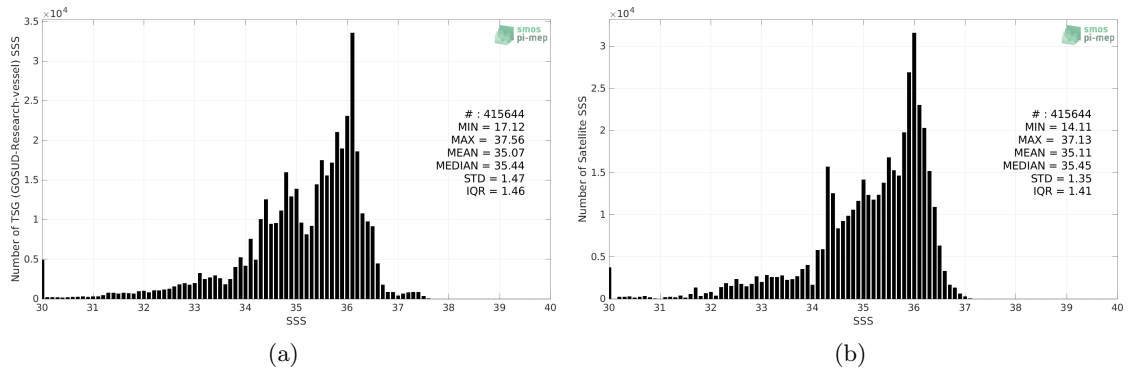
Figure 2: Histograms of SSS from TSG (GOSUD-Research-vessel) (a) and SMAP SSS L3 v4 - 8-Day running (RSS) (b) considering all match-up pairs per bins of 0.1 over the Equatorial Ocean 10N-10S Pi-MEP region and for the full satellite product period.
