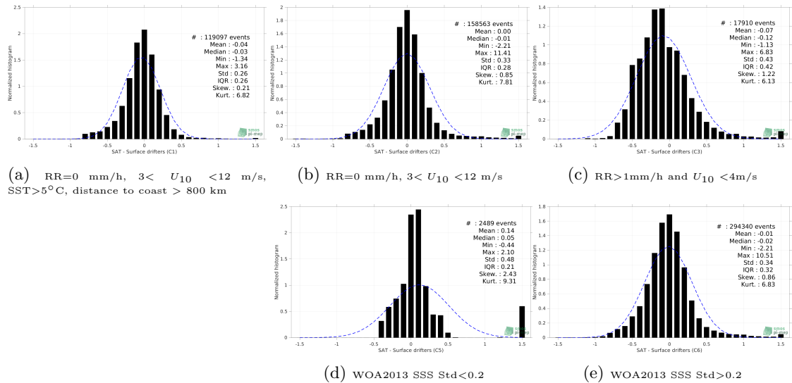
Figure 12: Normalized histogram of \Delta SSS (SMAP SSS L3 v4 - 8-Day running (RSS) - Surface drifters) for 5 different subdatasets corresponding to: RR=0 mm/h, 3 < U_{10} < 12 m/s, SST >5^\circ C, distance to coast > 800 km (a), RR=0 mm/h, 3 < U_{10} < 12 m/s (b), RR >1 mm/h and U_{10} < 4 m/s (c), WOA2013 SSS Std <0.2 (d), WOA2013 SSS Std >0.2 (e).
