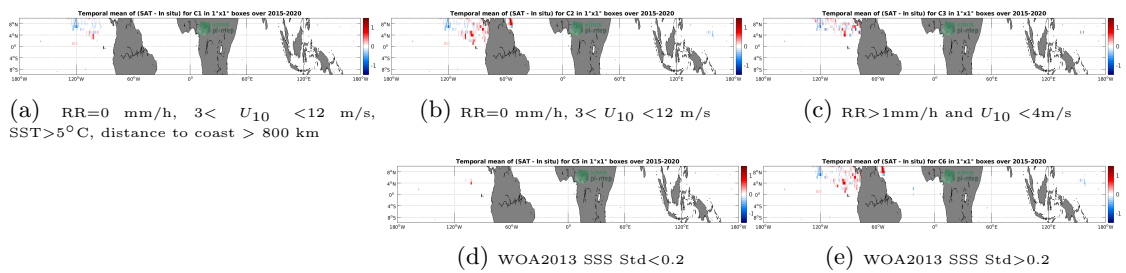
Figure 11: Temporal mean gridded over spatial boxes of size 1^\circ \times 1^\circ of \Delta SSS (SMAP SSS L3 v4 - 8-Day running (RSS) - Surface drifters) for 5 different subdatasets corresponding to:RR=0 mm/h, 3 < U_{10} < 12 m/s, SST>5°C, distance to coast > 800 km (a), RR=0 mm/h, 3 < U_{10} < 12 m/s (b), RR>1mm/h and U_{10} < 4 m/s (c), WOA2013 SSS Std<0.2 (d), WOA2013 SSS Std>0.2 (e).
