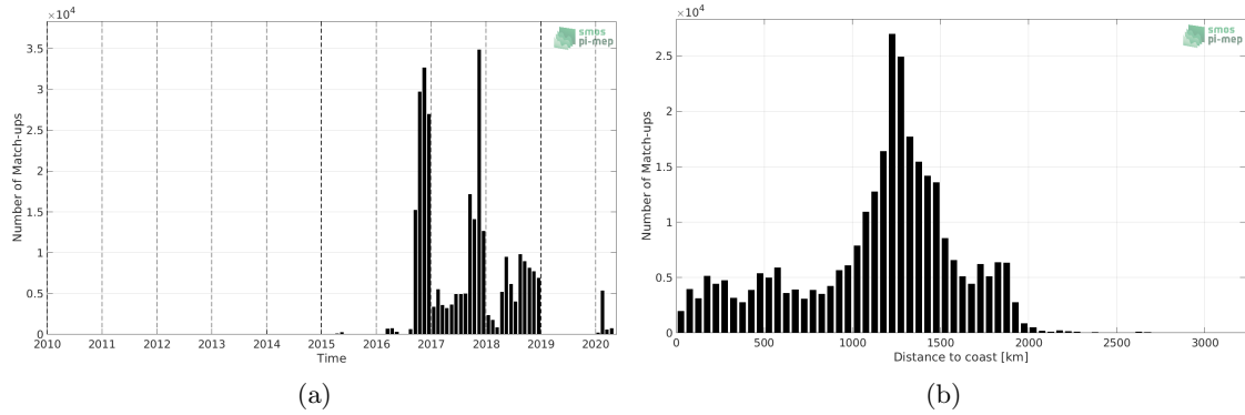
Figure 1: Number of match-ups between Surface drifters and SMAP SSS L3 v4 - 8-Day running (RSS) SSS as a function of time (a) and as function of the distance to coast (b) over the Equatorial Ocean 10N-10S Pi-MEP region and for the full satellite product period.
