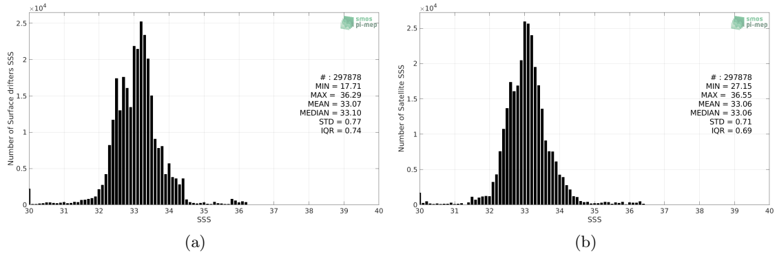
Figure 2: Histograms of SSS from Surface drifters (a) and SMAP SSS L3 v4 - 8-Day running (RSS) (b) considering all match-up pairs per bins of 0.1 over the Equatorial Ocean 10N-10S Pi-MEP region and for the full satellite product period.
