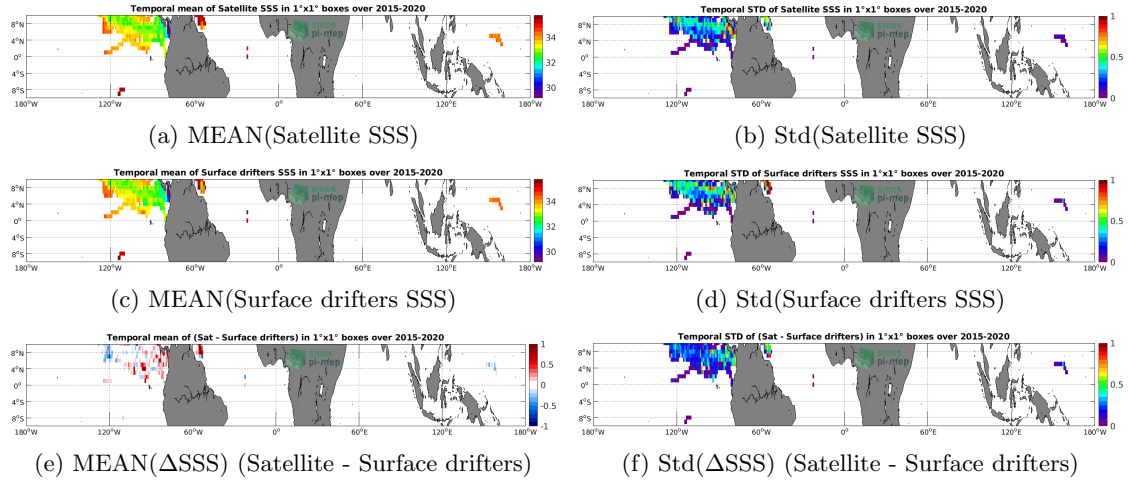
Figure 5: Temporal mean (left) and Std (right) of SSS from SMAP SSS L3 v4 - 8-Day running (RSS) (top), Surface drifters (middle), and of \Delta SSS (Satellite - Surface drifters). Only match-up pairs are used to generate these maps.
