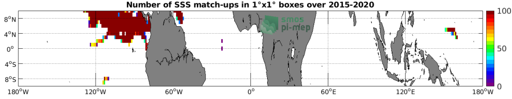
Figure 3: Number of SSS match-ups between Surface drifters SSS and the SMAP SSS L3 v4 - 8-Day running (RSS) SSS product for the Equatorial Ocean 10N-10S Pi-MEP region over 1^\circ \times 1^\circ boxes and for the full satellite product period.
