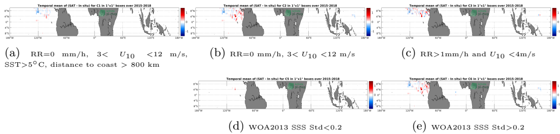
Figure 11: Temporal mean gridded over spatial boxes of size 1°x1° of \Delta SSS (SMAP SSS L3 v4 - 8-Day running (RSS) - Surface drifters) for 5 different subdatasets corresponding to:RR=0 mm/h, 3 < U_{10} < 12 m/s, SST>5°C, distance to coast > 800 km (a), RR=0 mm/h, 3 < U_{10} < 12 m/s (b), RR>1mm/h and U_{10} < 4m/s (c), WOA2013 SSS Std<0.2 (d), WOA2013 SSS Std>0.2 (e).
