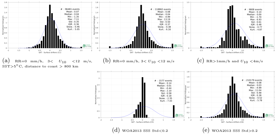
Figure 12: Normalized histogram of \Delta SSS (SMAP-L3-RSS-V4-8DAY-RUNNING - Surface drifters) for 5 different subdatasets corresponding to: RR=0 mm/h, 3 < U_{10} < 12 m/s, SST > 5^\circ\text{C} , distance to coast > 800 km (a), RR=0 mm/h, 3 < U_{10} < 12 m/s (b), RR > 1 mm/h and U_{10} < 4 m/s (c), WOA2013 SSS Std < 0.2 (d), WOA2013 SSS Std > 0.2 (e).
