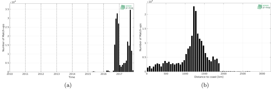
Figure 1: Number of match-ups between Surface drifters and SMAP-L3-RSS-V4-8DAY-RUNNING SSS as a function of time (a) and as function of the distance to coast (b) over the Equatorial Ocean 10N-10S Pi-MEP region and for the full satellite product period.
