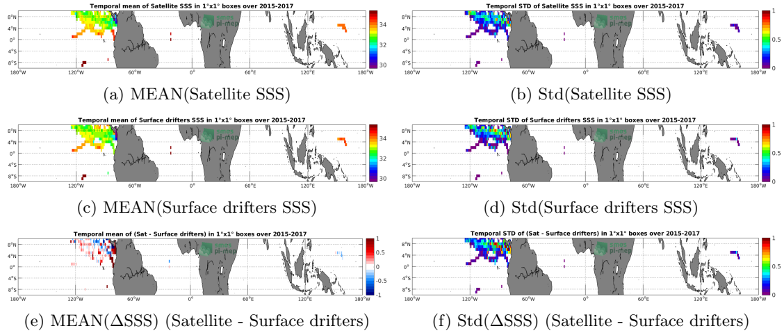
Figure 5: Temporal mean (left) and Std (right) of SSS from SMAP-L3-RSS-V4-8DAY-RUNNING (top), Surface drifters (middle), and of \Delta SSS (Satellite - Surface drifters). Only match-up pairs are used to generate these maps.
