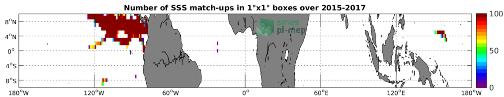
Figure 3: Number of SSS match-ups between Surface drifters SSS and the SMAP-L3-RSS-V4-8DAY-RUNNING SSS product for the Equatorial Ocean 10N-10S Pi-MEP region over 1°x1° boxes and for the full satellite product period.
