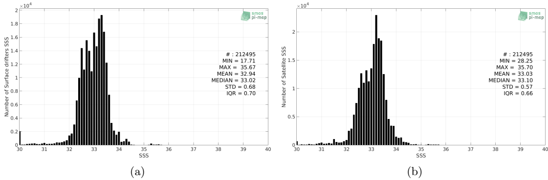
Figure 2: Histograms of SSS from Surface drifters (a) and SMAP-L3-RSS-V4-8DAY-RUNNING (b) considering all match-up pairs per bins of 0.1 over the Equatorial Ocean 10N-10S Pi-MEP region and for the full satellite product period.
