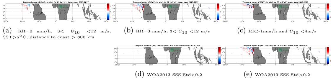
Figure 11: Temporal mean gridded over spatial boxes of size 1^\circ \times 1^\circ of \Delta SSS (SMAP-L3-RSS-V4-8DAY-RUNNING - Surface drifters) for 5 different subdatasets corresponding to: RR=0 mm/h, 3 < U_{10} < 12 m/s, SST > 5^\circ\text{C} , distance to coast > 800 km (a), RR=0 mm/h, 3 < U_{10} < 12 m/s (b), RR > 1 mm/h and U_{10} < 4 m/s (c), WOA2013 SSS Std < 0.2 (d), WOA2013 SSS Std > 0.2 (e).
