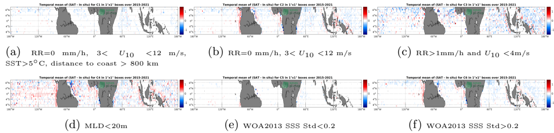
Figure 12: Temporal mean gridded over spatial boxes of size 1^\circ \times 1^\circ of \Delta SSS (SMAP SSS L3 v4 - 8-Day running (RSS) - Argo) for 6 different subdatasets corresponding to:RR=0 mm/h, 3 < U_{10} < 12 m/s, SST > 5^\circ C , distance to coast > 800 km (a), RR=0 mm/h, 3 < U_{10} < 12 m/s (b), RR > 1 mm/h and U_{10} < 4 m/s (c),MLD < 20 m (d),WOA2013 SSS Std < 0.2 (e),WOA2013 SSS Std > 0.2 (f).
