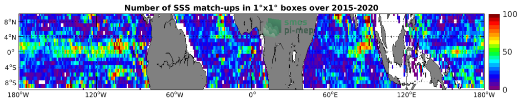
Figure 4: Number of SSS match-ups between Argo SSS and the SMAP SSS L3 v4 - 8-Day running (RSS) SSS product for the Equatorial Ocean 10N-10S Pi-MEP region over 1°x1° boxes and for the full satellite product period.
