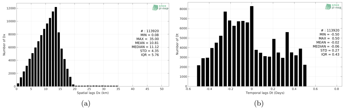
Figure 5: Histograms of the spatial (a) and temporal (b) lags between the time of the Argos measurements and the date of the corresponding SMAP-L3-RSS-V4-8DAY-RUNNING SSS product.
