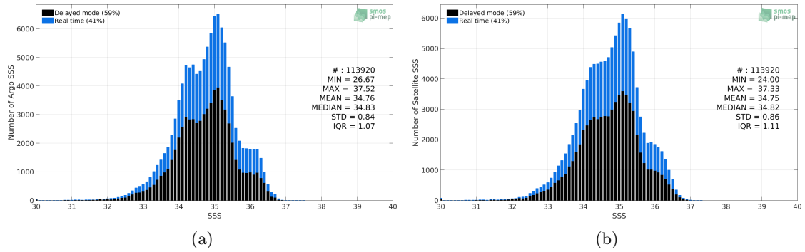
Figure 2: Histograms of SSS from Argo (a) and SMAP-L3-RSS-V4-8DAY-RUNNING (b) considering all match-up pairs per bins of 0.1 over the Equatorial Ocean 10N-10S Pi-MEP region and for the full satellite product period.
