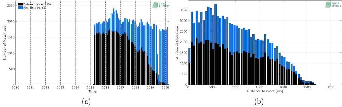
Figure 1: Number of match-ups between Argo and SMAP-L3-RSS-V4-8DAY-RUNNING SSS as a function of time (a) and as function of the distance to coast (b) over the Equatorial Ocean 10N-10S Pi-MEP region and for the full satellite product period.
