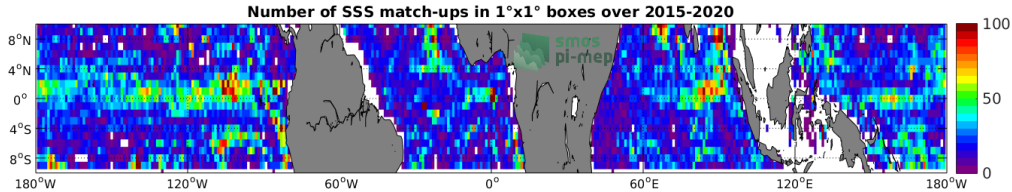
Figure 4: Number of SSS match-ups between Argos SSS and the SMAP-L3-RSS-V4-8DAY-RUNNING SSS product for the Equatorial Ocean 10N-10S Pi-MEP region over 1°x1° boxes and for the full satellite product period.
