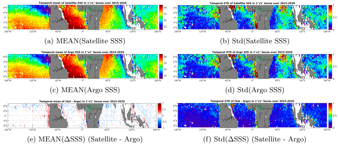
Figure 6: Temporal mean (left) and Std (right) of SSS from SMAP-L3-RSS-V4-8DAY-RUNNING (top), Argo (middle), and of \Delta SSS (Satellite - Argo). Only match-up pairs are used to generate these maps.
