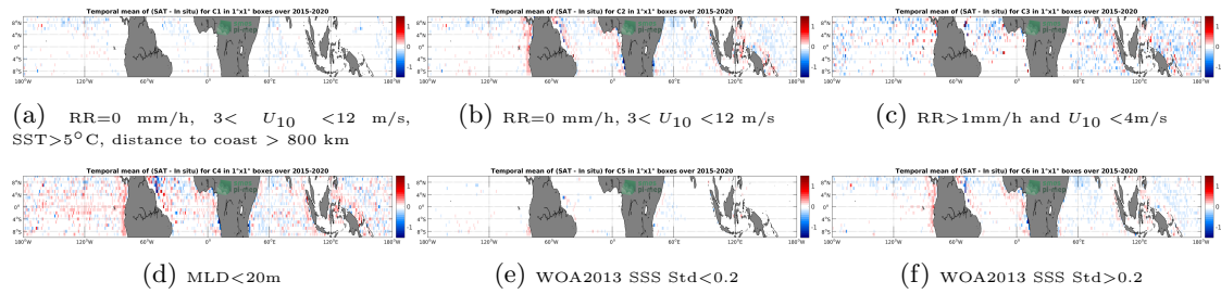
Figure 12: Temporal mean gridded over spatial boxes of size 1^\circ \times 1^\circ of \Delta SSS (SMAP-L3-RSS-V4-8DAY-RUNNING - Argo) for 6 different subdatasets corresponding to:RR=0 mm/h, 3 < U_{10} < 12 m/s, SST >5^\circ\text{C} , distance to coast > 800 km (a), RR=0 mm/h, 3 < U_{10} < 12 m/s (b), RR >1 mm/h and U_{10} < 4 m/s (c),MLD <20 m (d),WOA2013 SSS Std <0.2 (e),WOA2013 SSS Std >0.2 (f).
