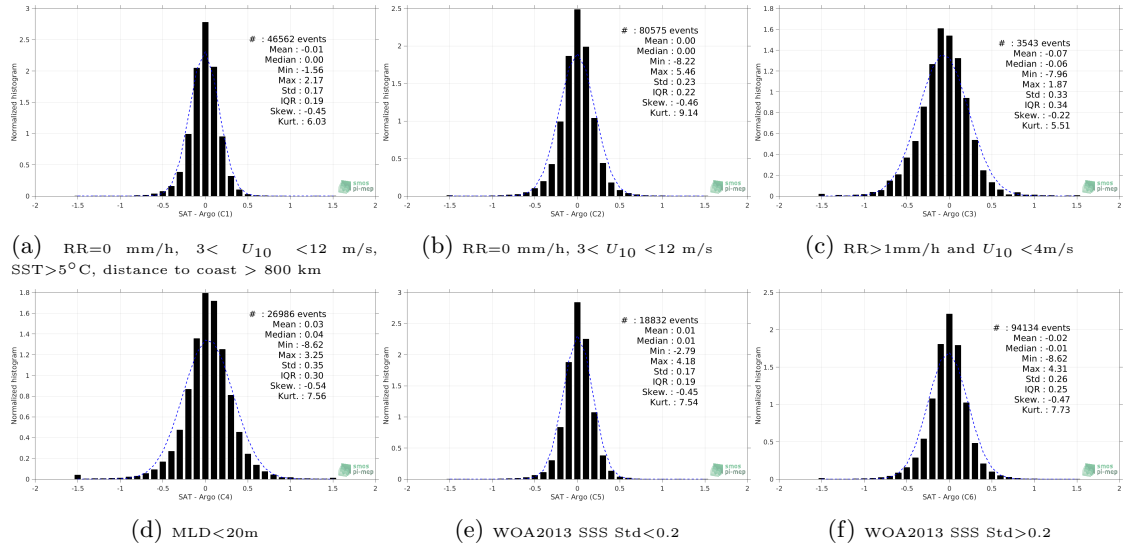
Figure 13: Normalized histogram of \Delta SSS (SMAP-L3-RSS-V4-8DAY-RUNNING - Argo) for 6 different subdatasets corresponding to: RR=0 mm/h, 3 < U_{10} < 12 m/s, SST >5^\circ\text{C} , distance to coast > 800 km (a), RR=0 mm/h, 3 < U_{10} < 12 m/s (b), RR >1 mm/h and U_{10} < 4 m/s (c), MLD <20 m (d), WOA2013 SSS Std <0.2 (e), WOA2013 SSS Std >0.2 (f).
